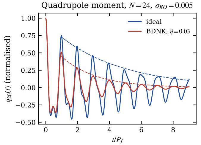
FIG. 1. The \ell = 2 quadrupole moment q_{20}(t) of the benchmark star at N = 24 , \sigma_{\text{KO}} = 0.005 , for the ideal engine and for BDNK in frame F_1 at \hat{\eta} = 0.03 , each normalised to its seed. Dashed: exponential fits to the positive peaks. The ideal run decays at the numerical floor \gamma_0 (Kreiss–Oliger dissipation and the surface); the viscous damping is the difference. The first half-period is the seed relaxing onto the mode.
