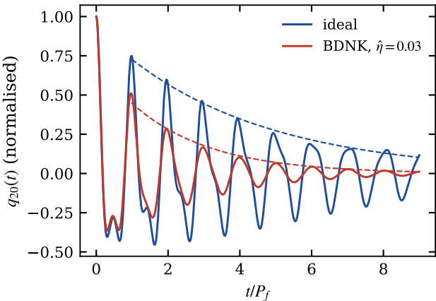
Quadrupole moment, N=24 , \sigma_{KO}=0.005
