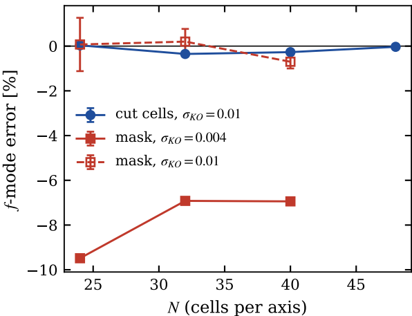
\ell = 2 f -mode vs shooting solver
