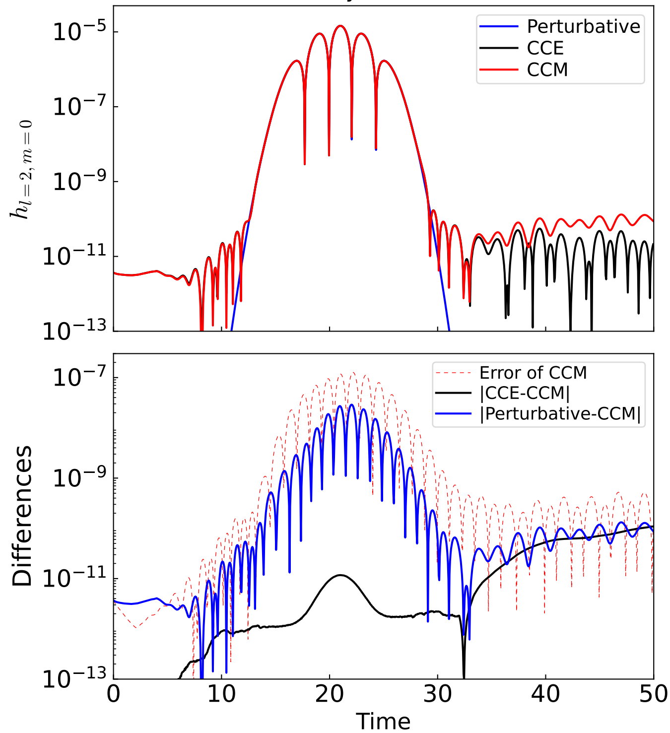
Teukolsky Wave X = 10^{-5}
