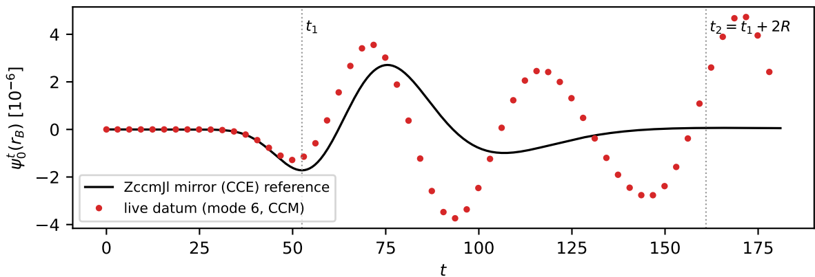
(a) Sec. V.C pulse: transparent (live CCM) vs mirror (quiescent-BC) worldtube
