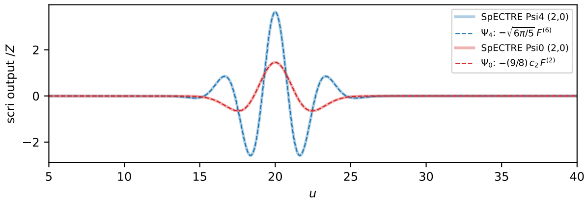
(c) SpECTRE CharacteristicExtract on the exact worldtube data vs the admitted closed forms
