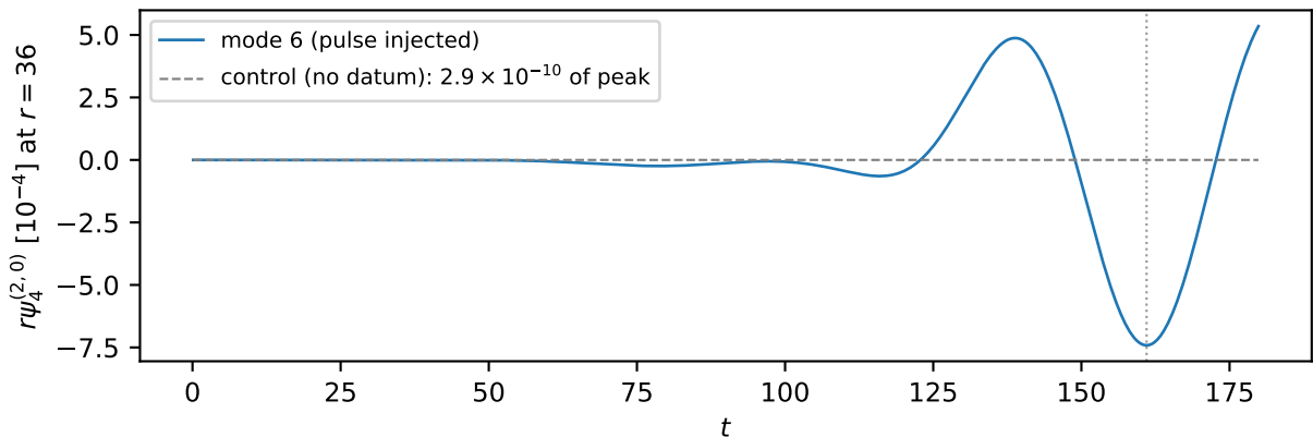
(b) the burst is transmitted through the Cauchy domain and exits at t_2
