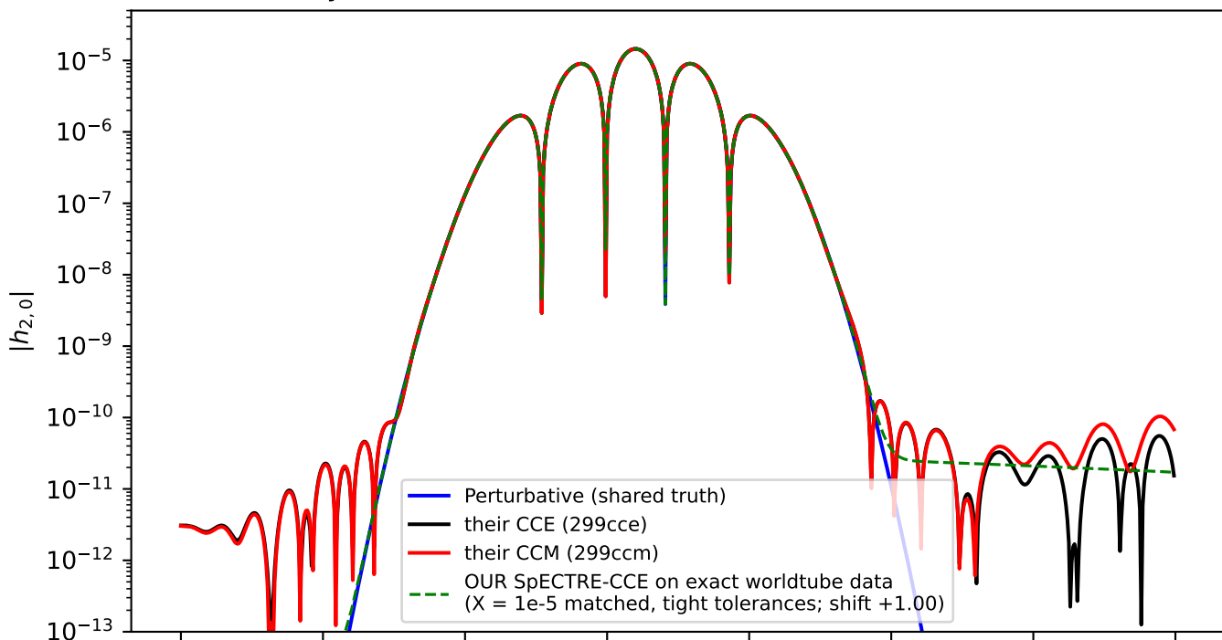
Teukolsky wave X = 10^{-5} , worldtube 41: scri strain, theirs vs ours
