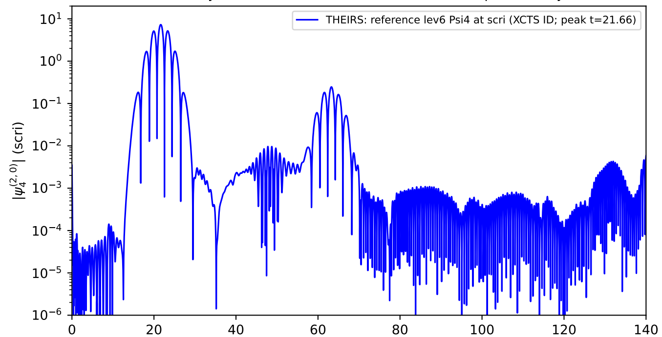
Teukolsky X=2: theirs vs ours — STRUCTURAL comparison only
