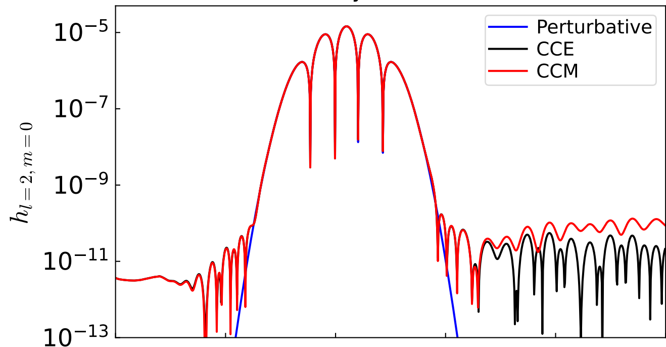
Teukolsky Wave X = 10^{-5}
