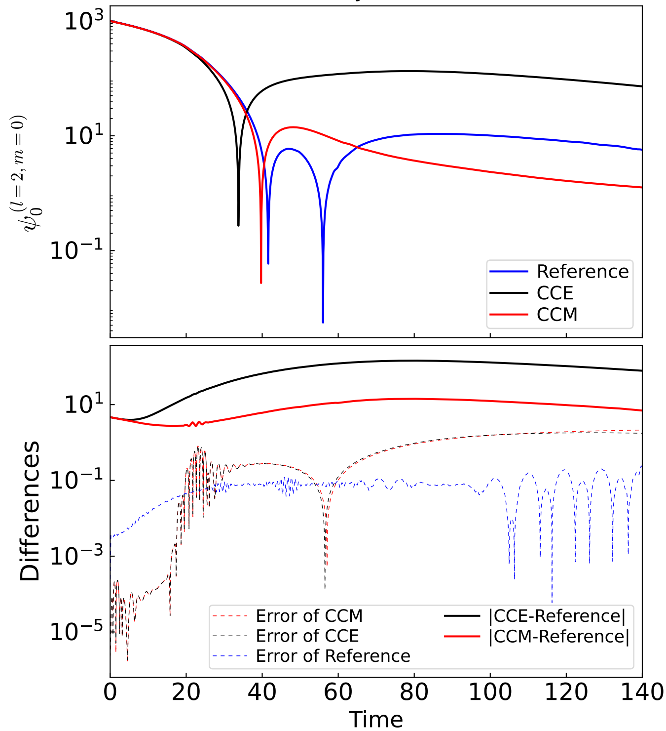
Teukolsky Wave X=2
