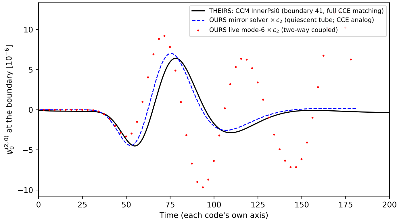
transmitted burst: their scri waveform vs our finite-radius extraction (feature offsets +2..+4 = tube 41 vs 40 geometry)
