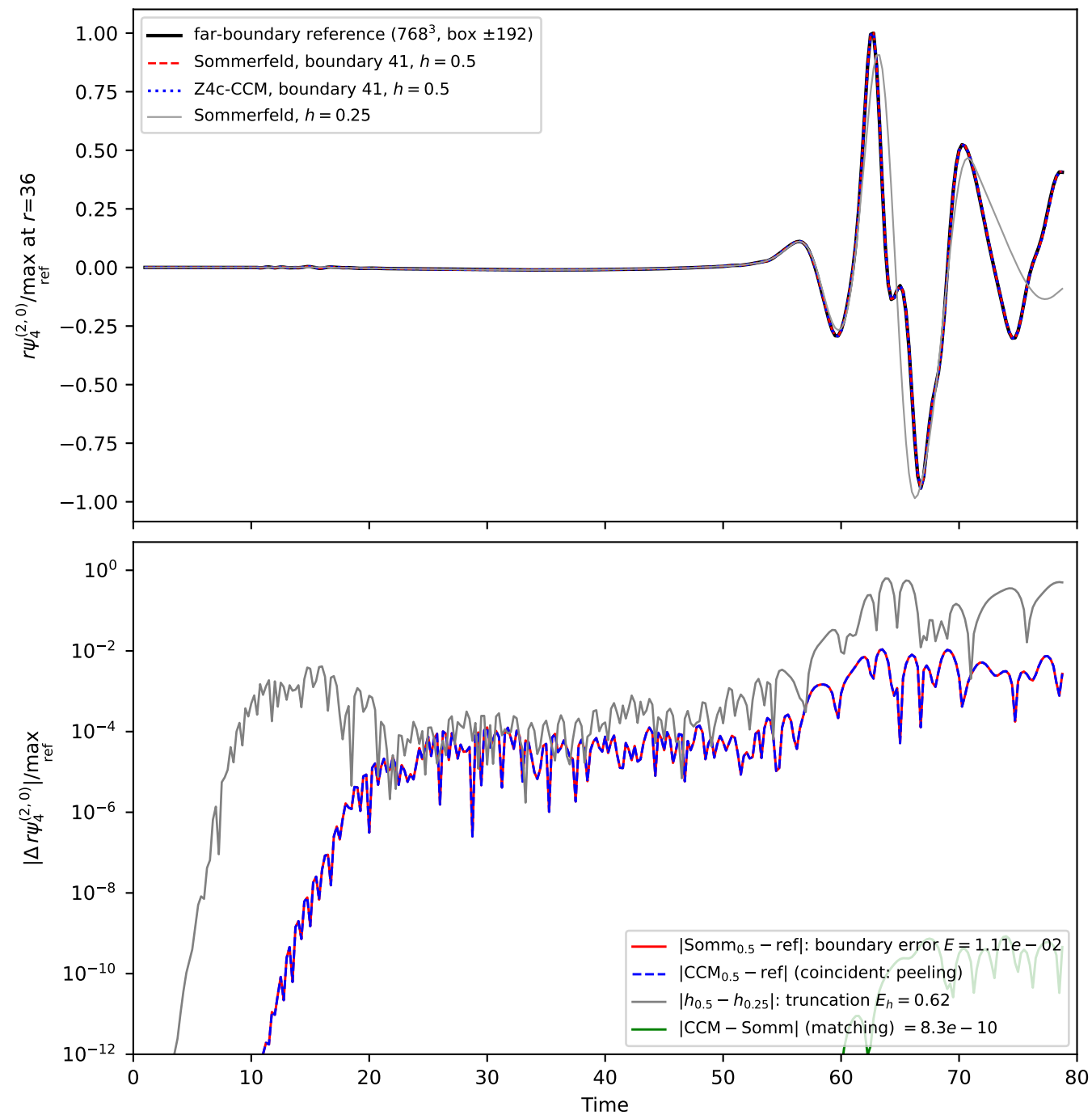
Teukolsky X = 2 : boundary-41 runs vs.\ the far-boundary reference
