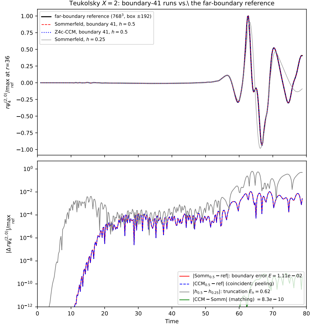
Figure 6. X = 2 error hierarchy from the dedicated eight-GPU campaign, all runs at the stable configuration (diss. 0.1, \kappa_1 = 0.1 , nghost = 4, t = 80 ). Top: r\psi_4^{(2,0)} at r = 36 for the causally disconnected far-boundary reference (768 3 , box \pm 192 ) and the boundary-41 Sommerfeld and Z4c-CCM runs at h = 0.5 (which track the reference) together with the h = 0.25 Sommerfeld run (whose late-time departure is the truncation effect). Bottom: at fixed resolution the boundary error |\text{run} - \text{ref}| is E = 1.1 \times 10^{-2} , identical for Sommerfeld and CCM; the matching-term difference |\text{CCM} - \text{Somm}| sits at 8 \times 10^{-10} (peeling); and the truncation estimate E_h = |h_{0.5} - h_{0.25}| reaches 0.6 — the boundary error lies far below the truncation error and is insensitive to the matching term, the X = 2 result of Ref. [1] reproduced with a shared linear-initial-data protocol. Generator: scripts/plot_x2_structural.py ; data: results/numerical/ccm_repro_x2_full .
