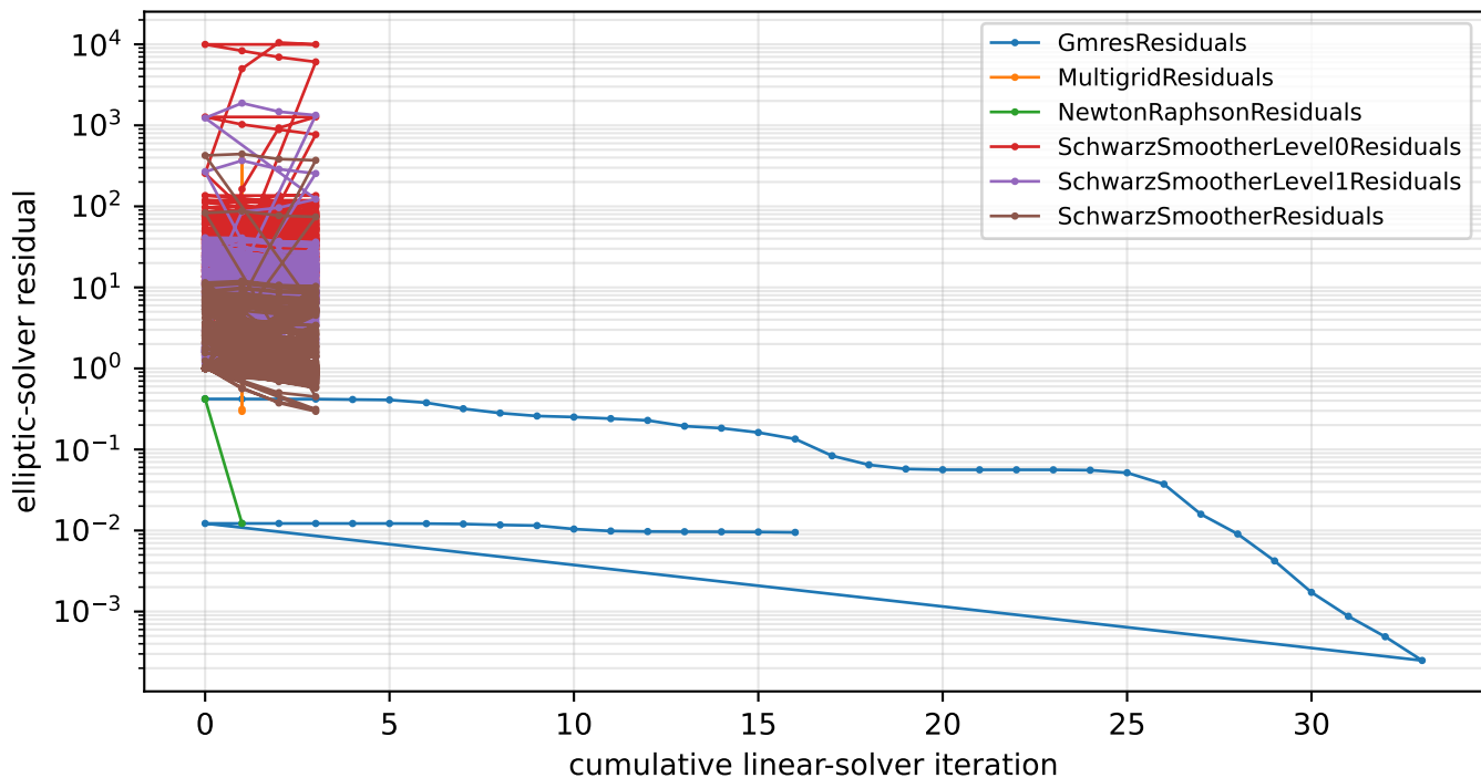
XCTS solve for the Teukolsky X = 2 free data: elliptic convergence
