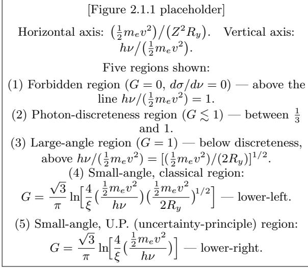
FIG. 1. Regions and Gaunt factors for bremsstrahlung of frequency \nu emitted by an electron of kinetic energy \frac{1}{2}m_e v^2 when it impinges on an ion of charge Ze .
