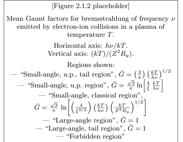
FIG. 2. Figure 2.1.2. Mean Gaunt factors for bremsstrahlung of frequency \nu emitted by electron-ion collisions in a plasma of temperature T .
