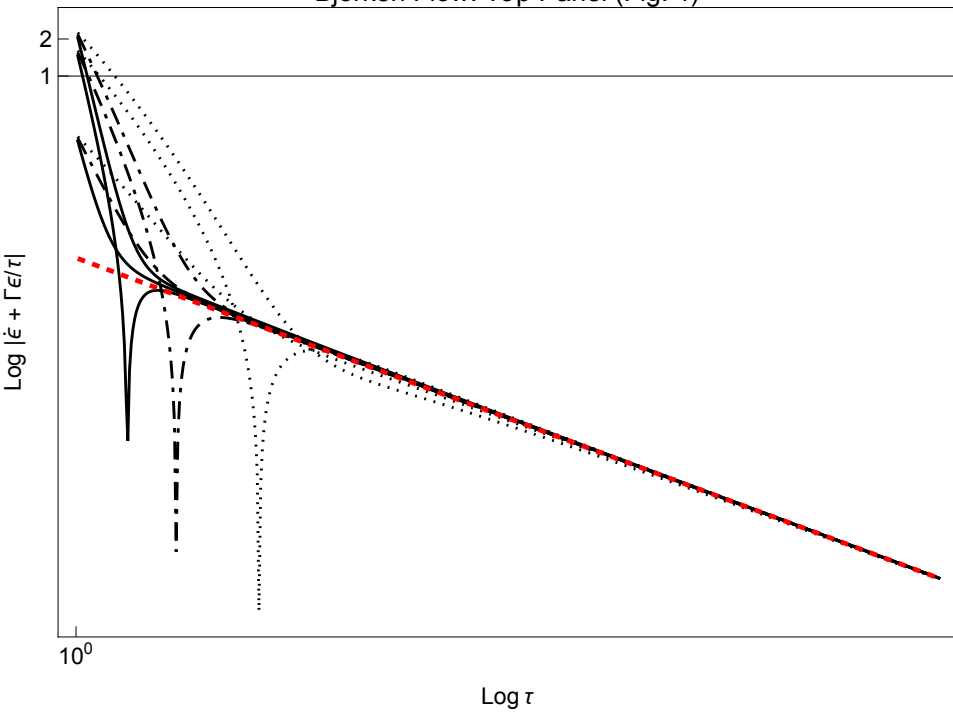
Bjorken Flow: Top Panel (Fig. 1)
