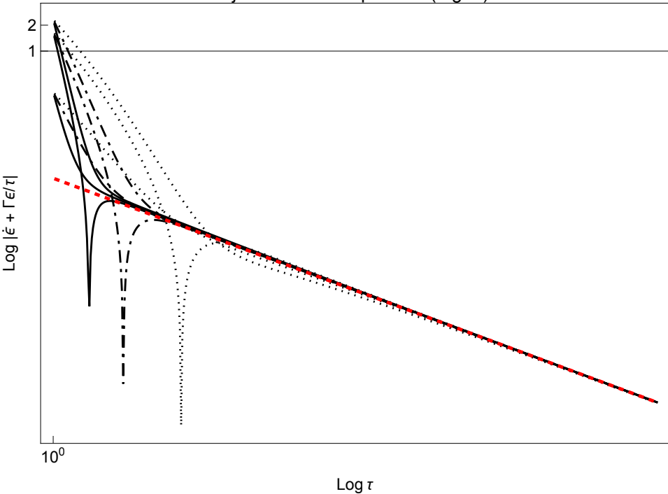
Bjorken Flow: Top Panel (Fig. 1)
