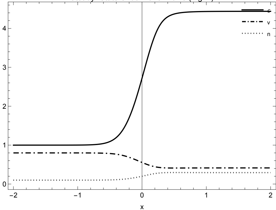
Steady-State Shockwave Profile (Fig. 2)
