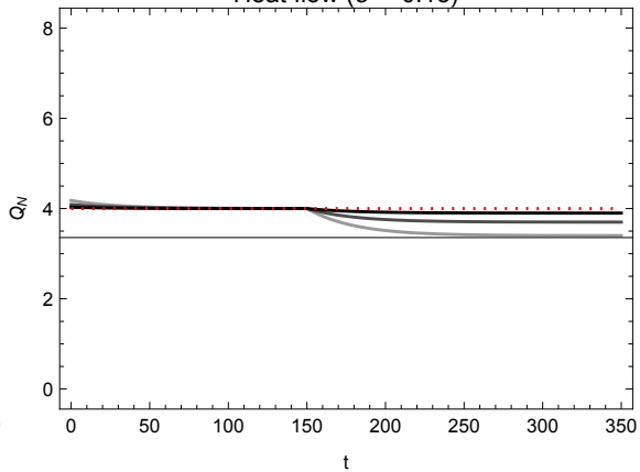
Heat flow ( \hat{\sigma} = 0.15 )
