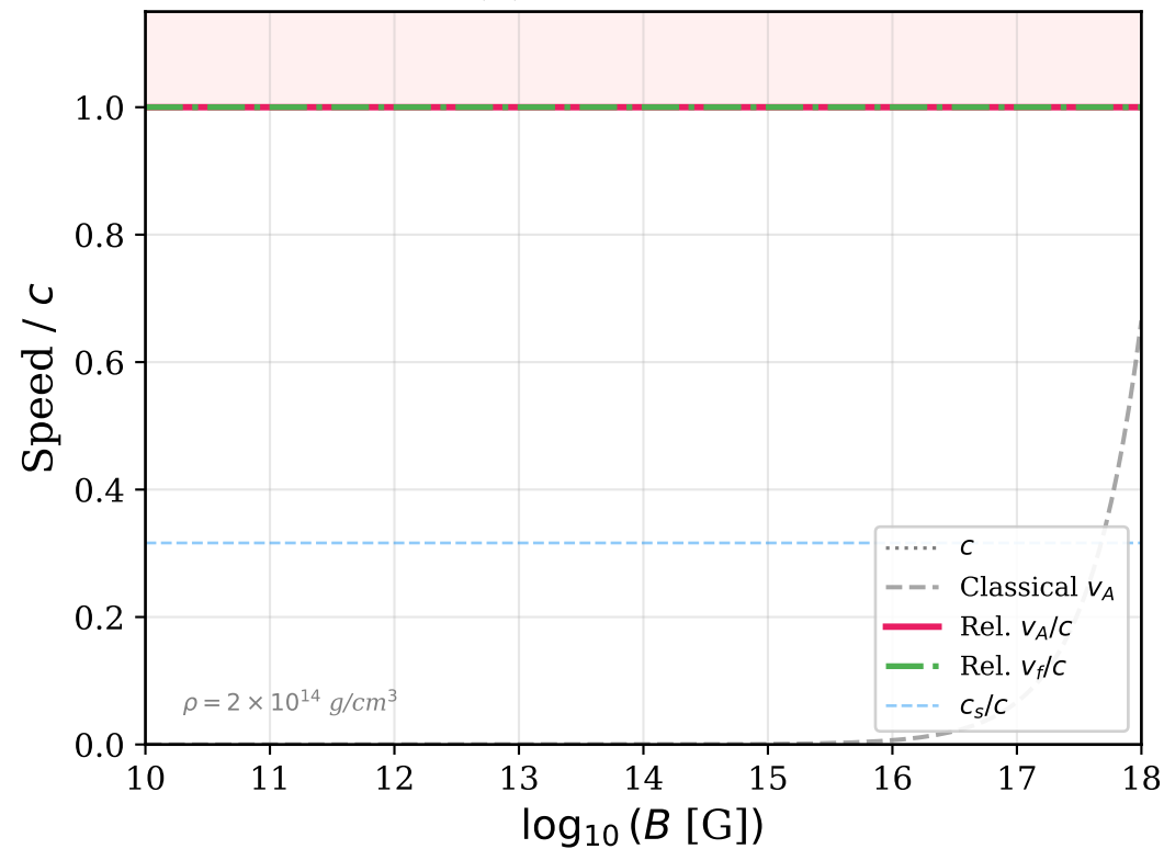
(a) Neutron Star
