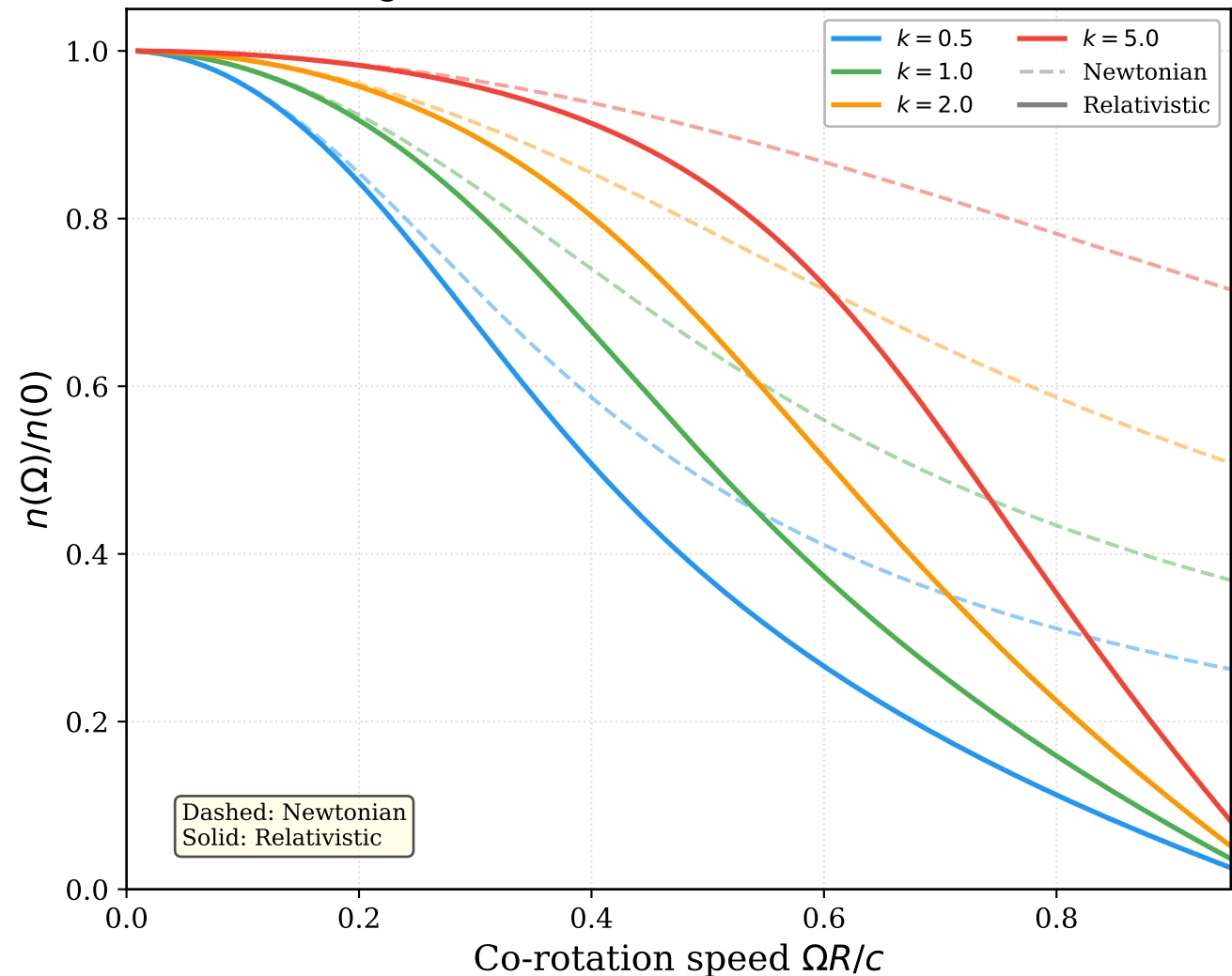
Centrifugal stabilization: Newtonian vs relativistic
