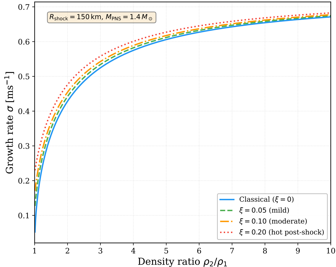
RT growth rate in core-collapse supernovae
