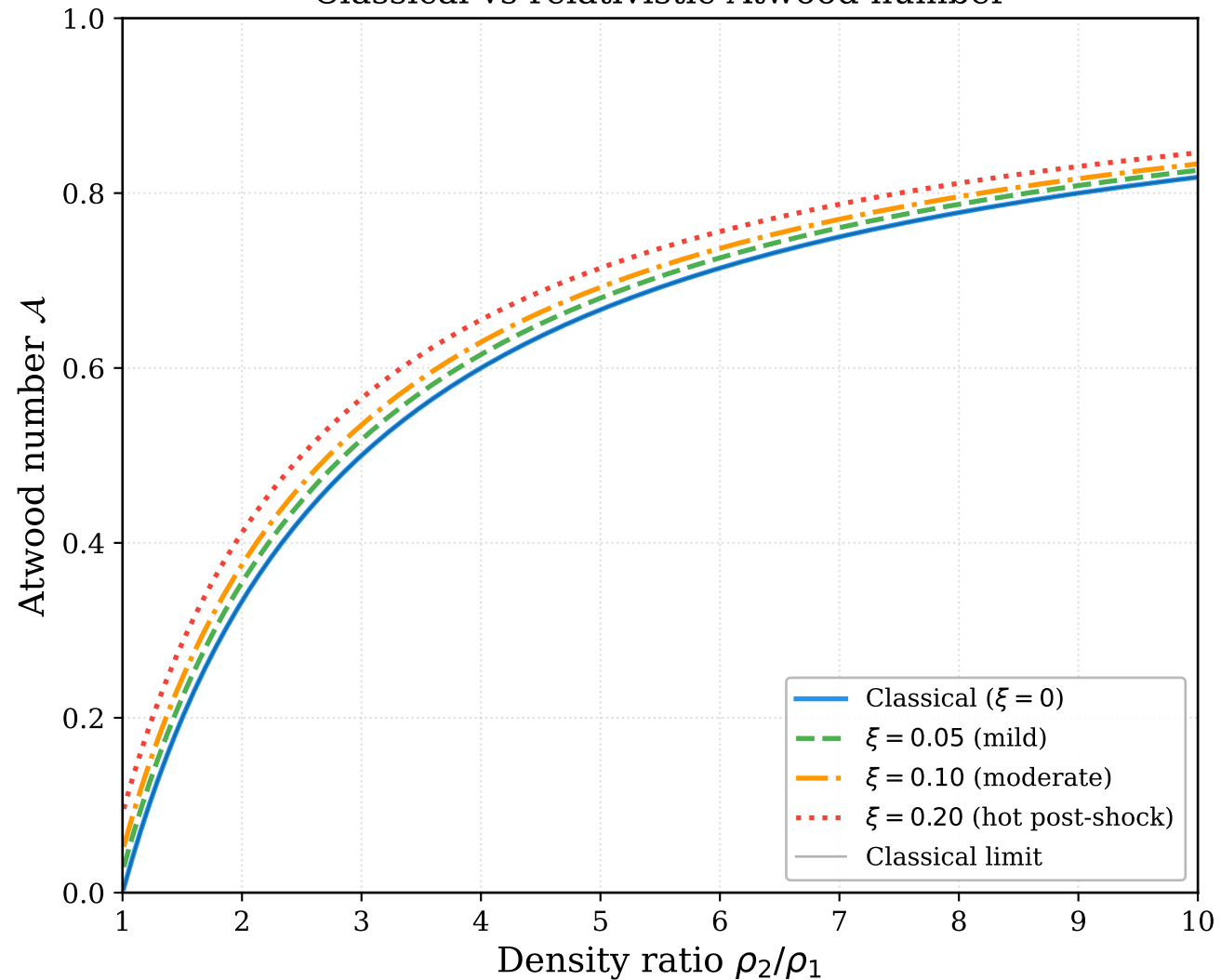
Classical vs relativistic Atwood number
