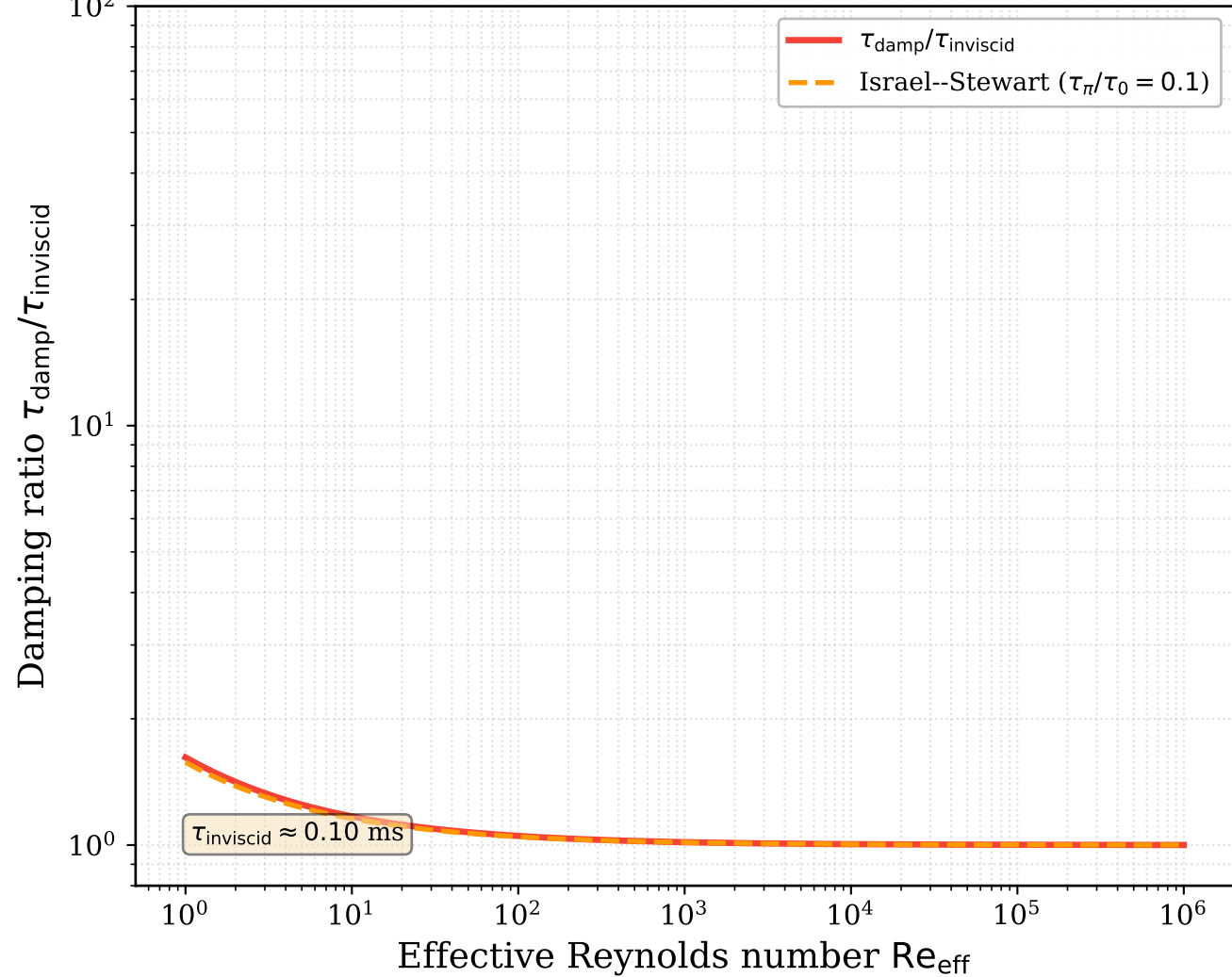
Viscous damping timescale (NS merger)
