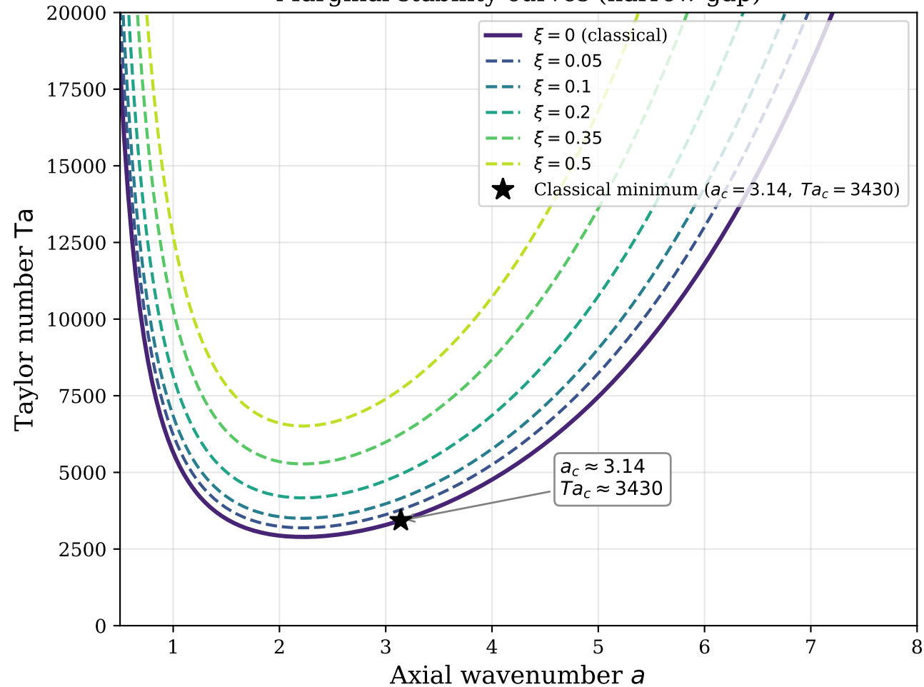
Marginal stability curves (narrow gap)
