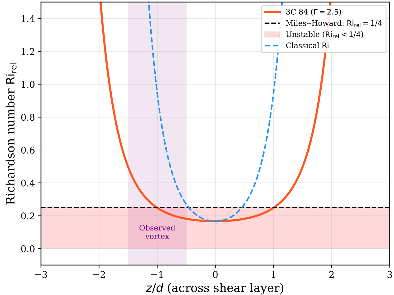
3C 84: Richardson number profile
