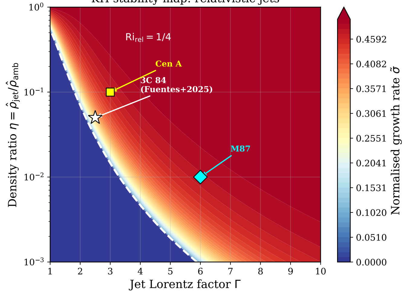
KH stability map: relativistic jets
