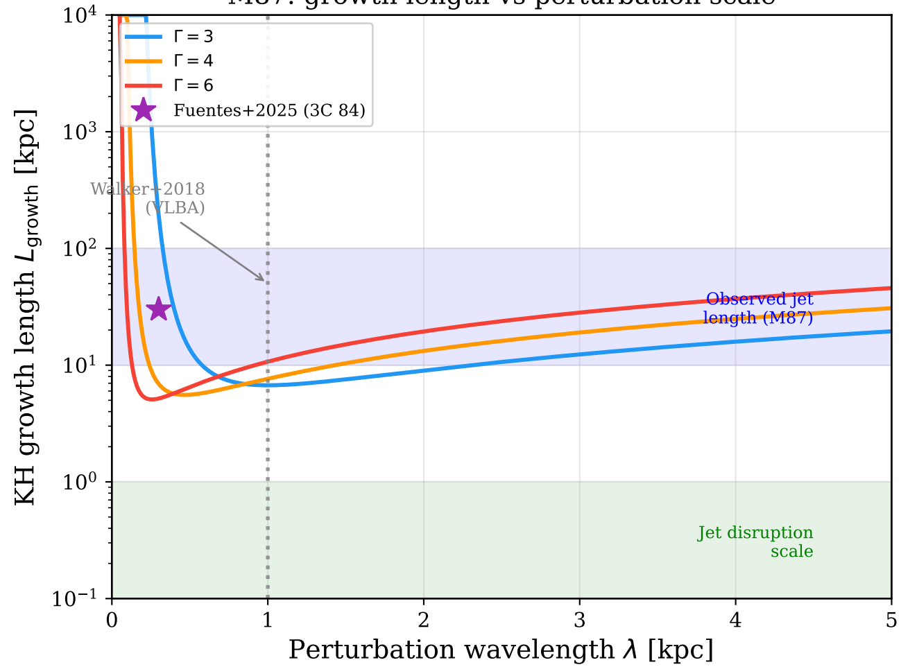
M87: growth length vs perturbation scale
