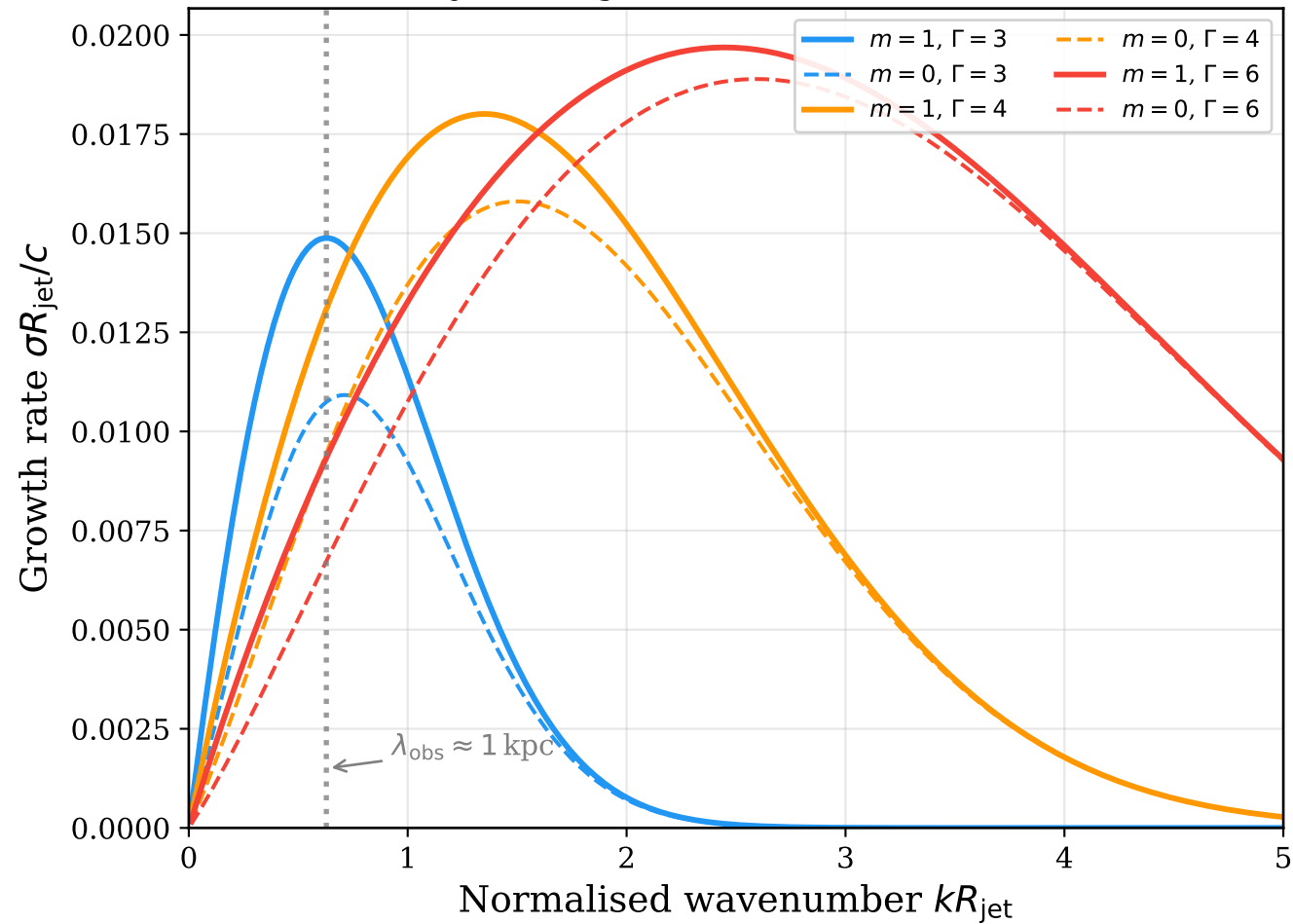
M87 jet: KH growth rate vs wavenumber
