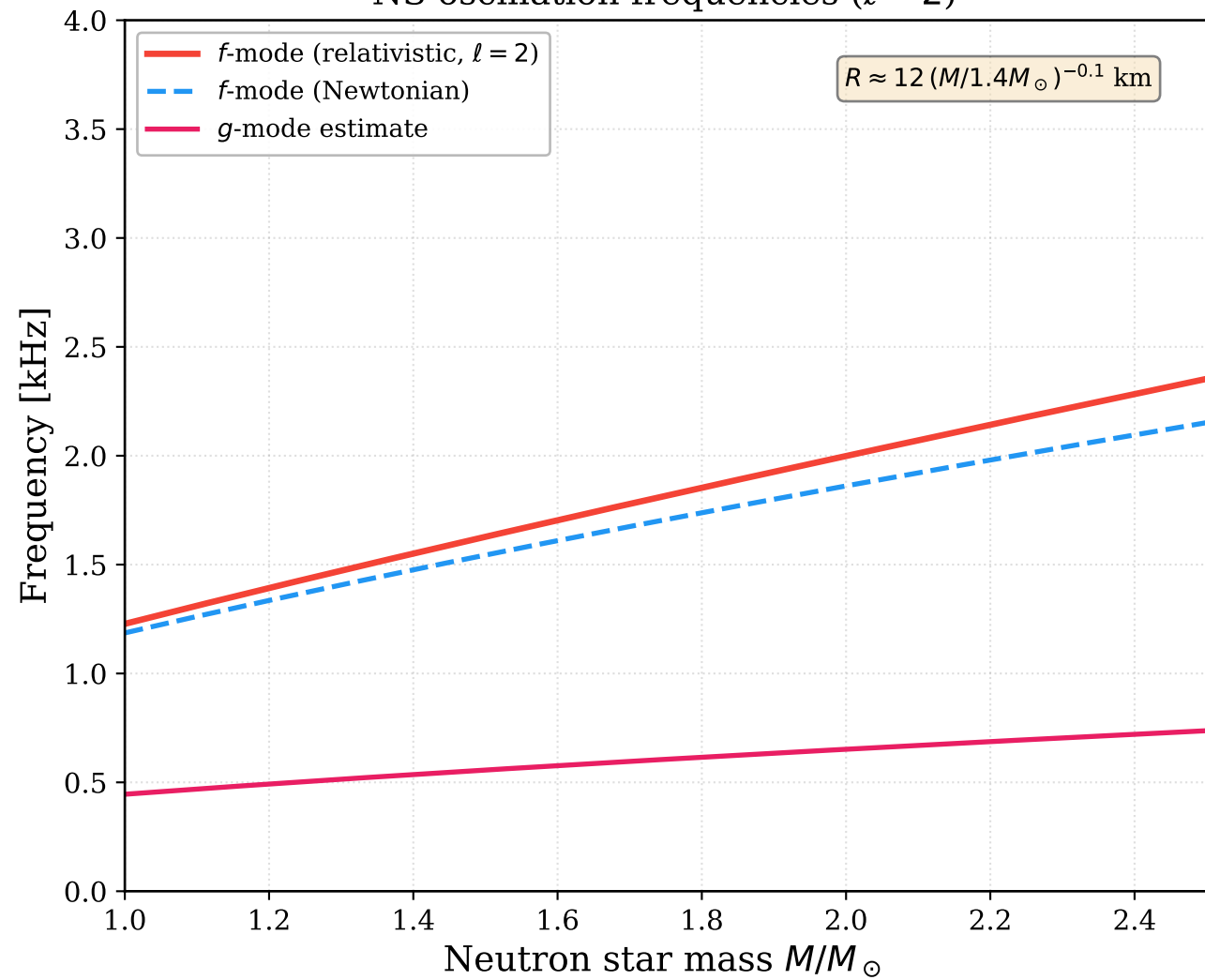
NS oscillation frequencies ( \ell = 2 )
