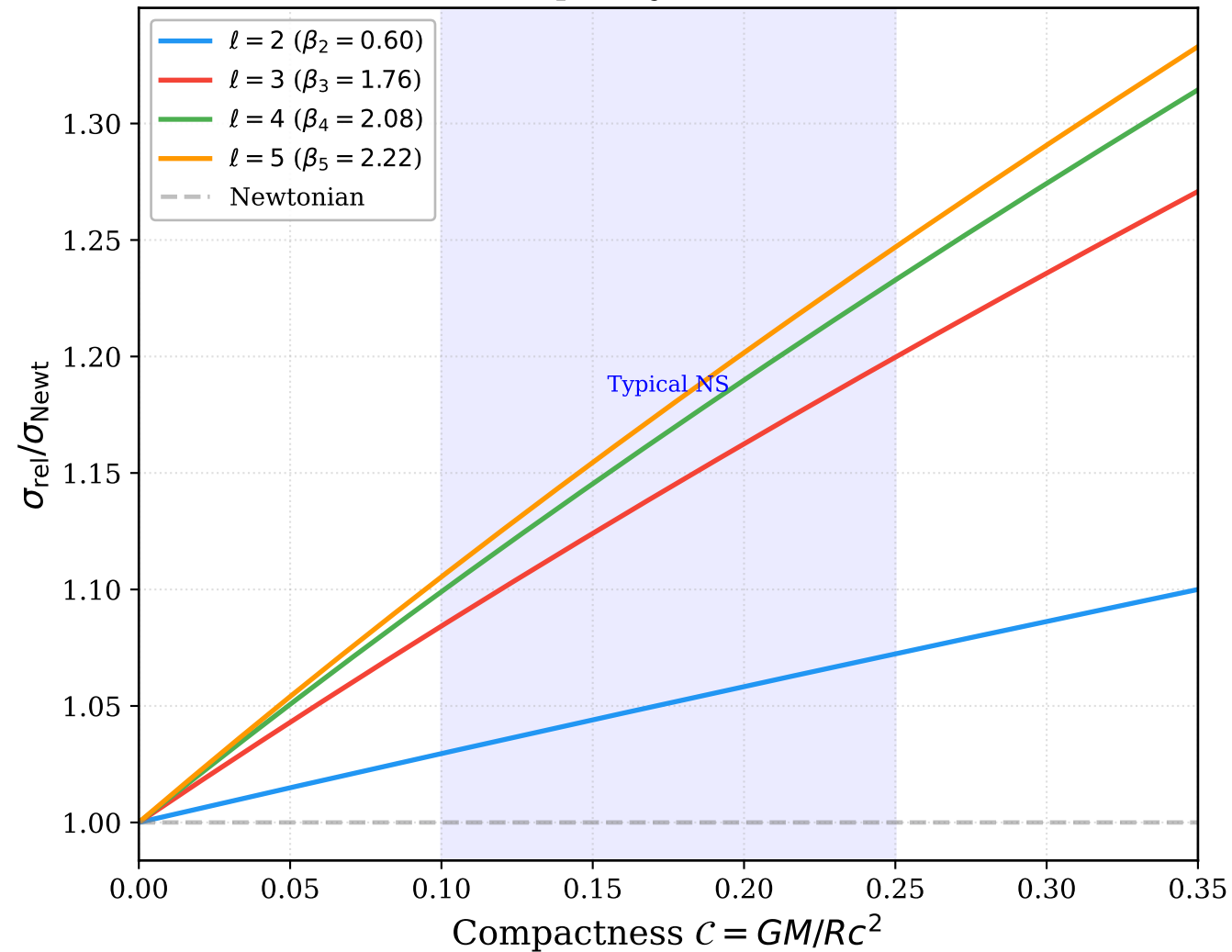
Kelvin mode frequency: relativistic correction
