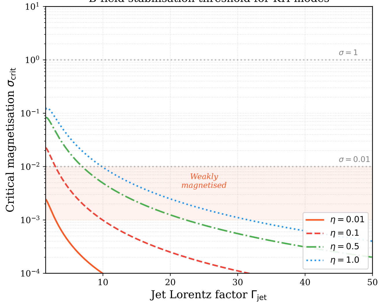
B-field stabilisation threshold for KH modes
