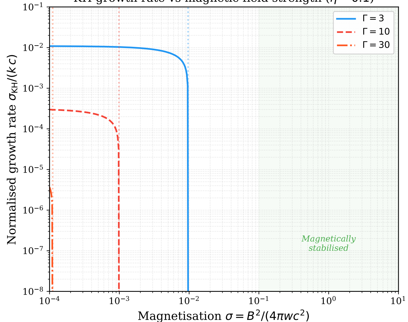
KH growth rate vs magnetic field strength ( \eta = 0.1 )
