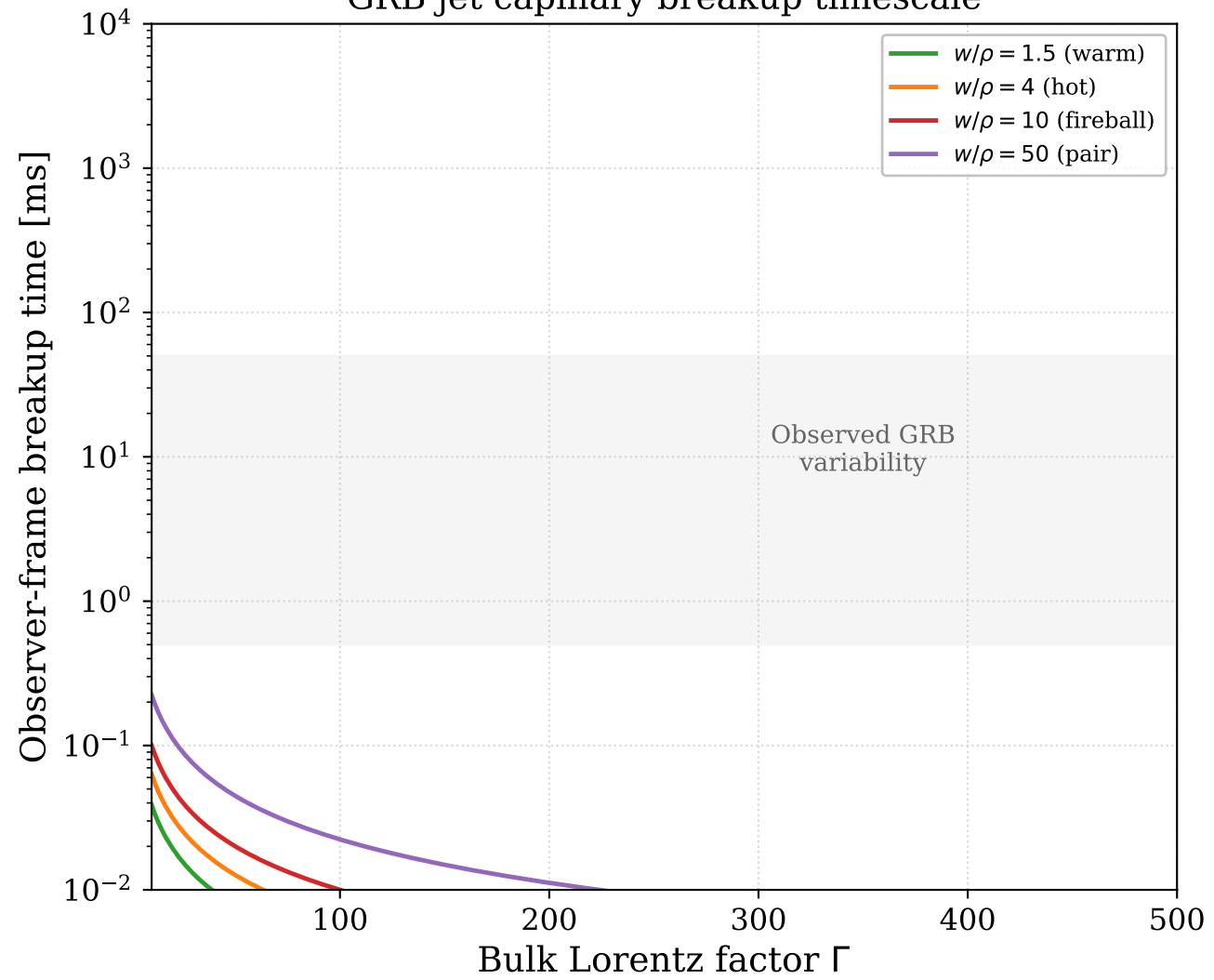
GRB jet capillary breakup timescale
