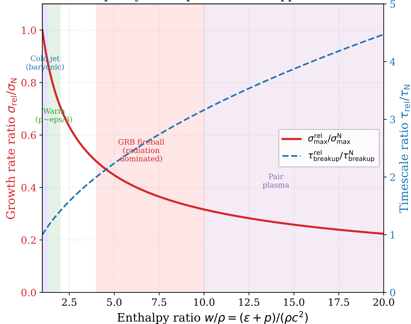
Capillary breakup: relativistic suppression
