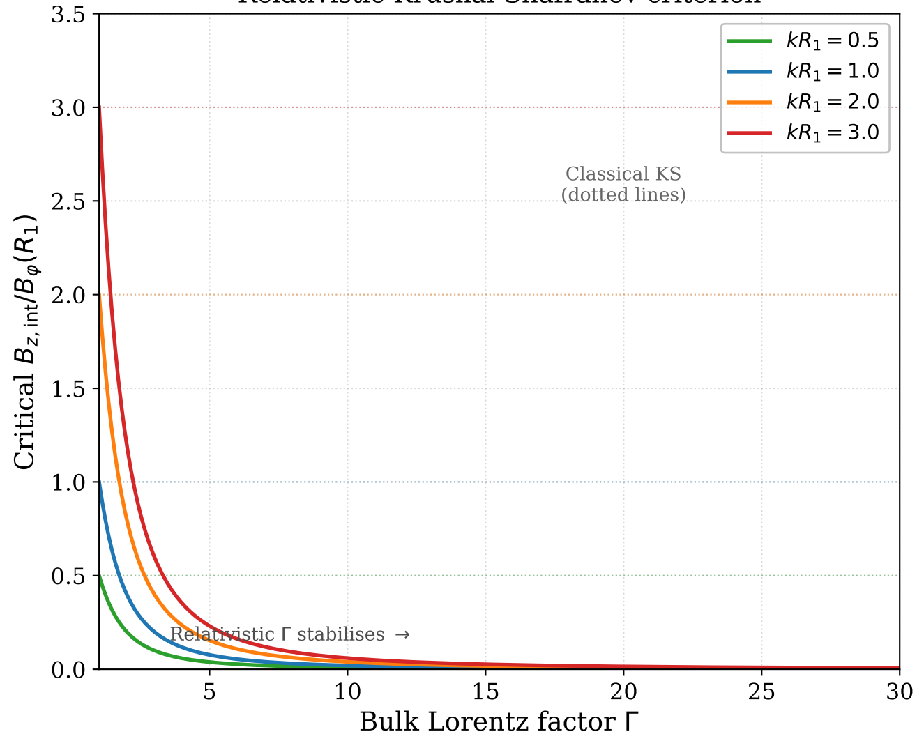
Relativistic Kruskal-Shafranov criterion
