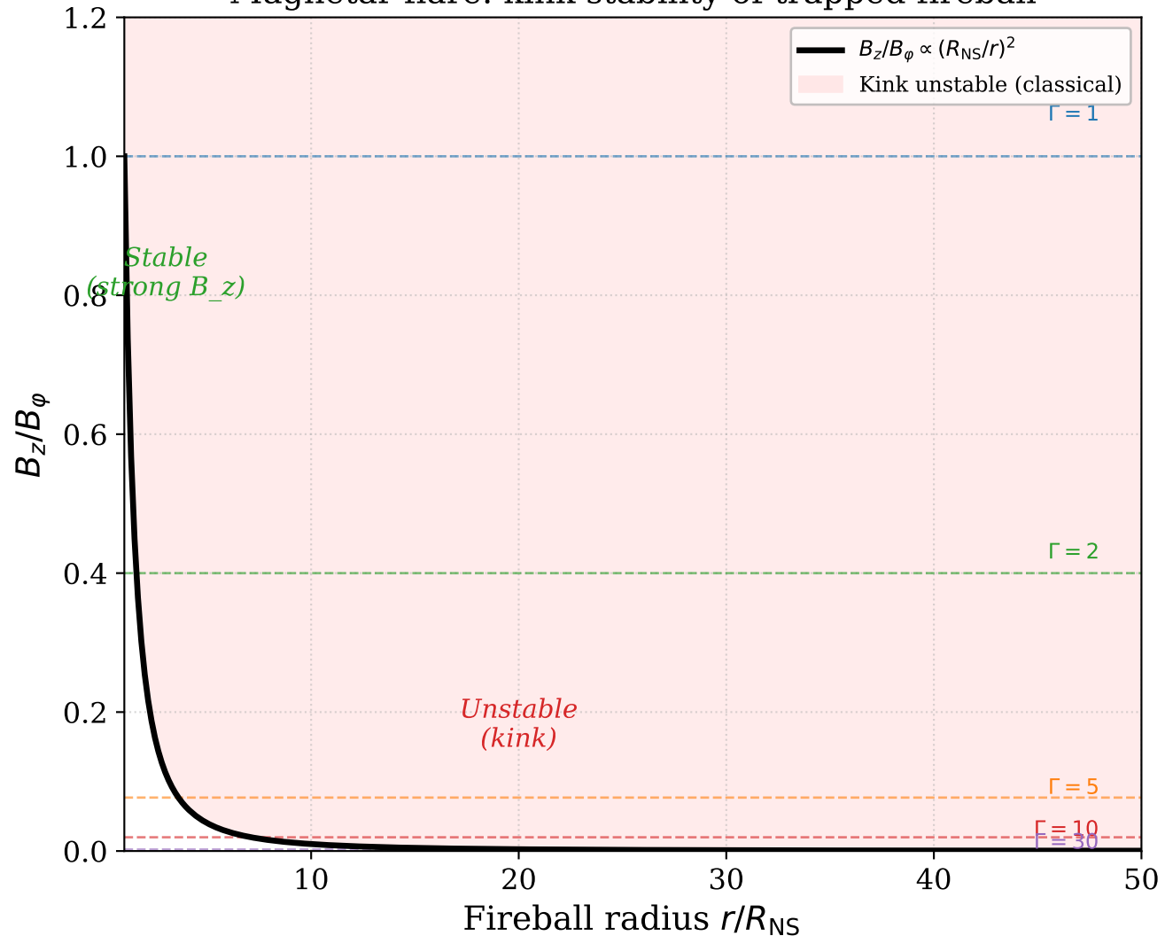
Magnetar flare: kink stability of trapped fireball
