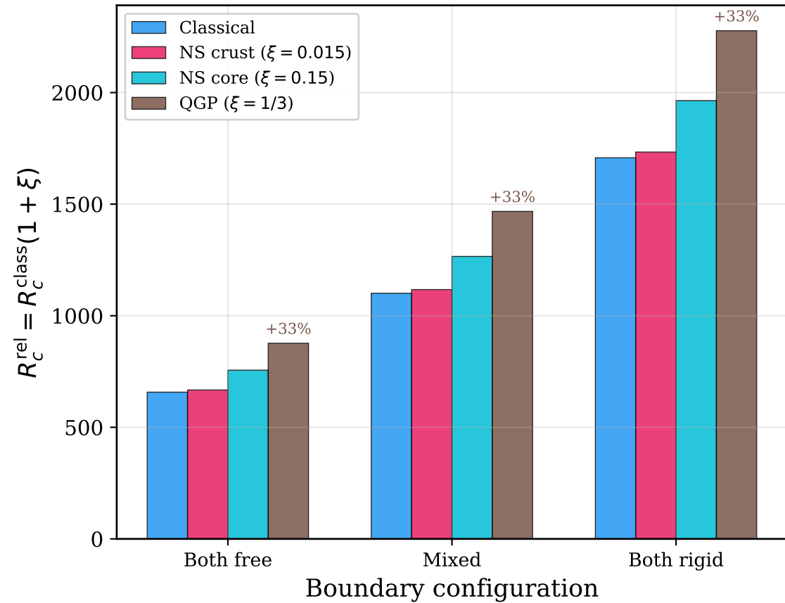
(a) Critical Rayleigh numbers
