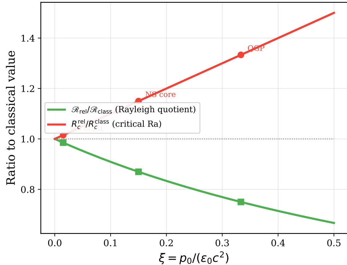
(a) Relativistic modification of Rayleigh quotient
