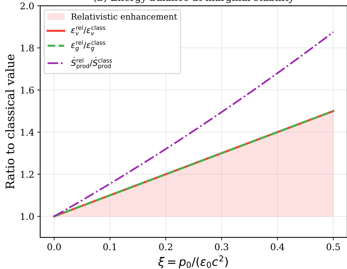
(b) Energy balance at marginal stability
