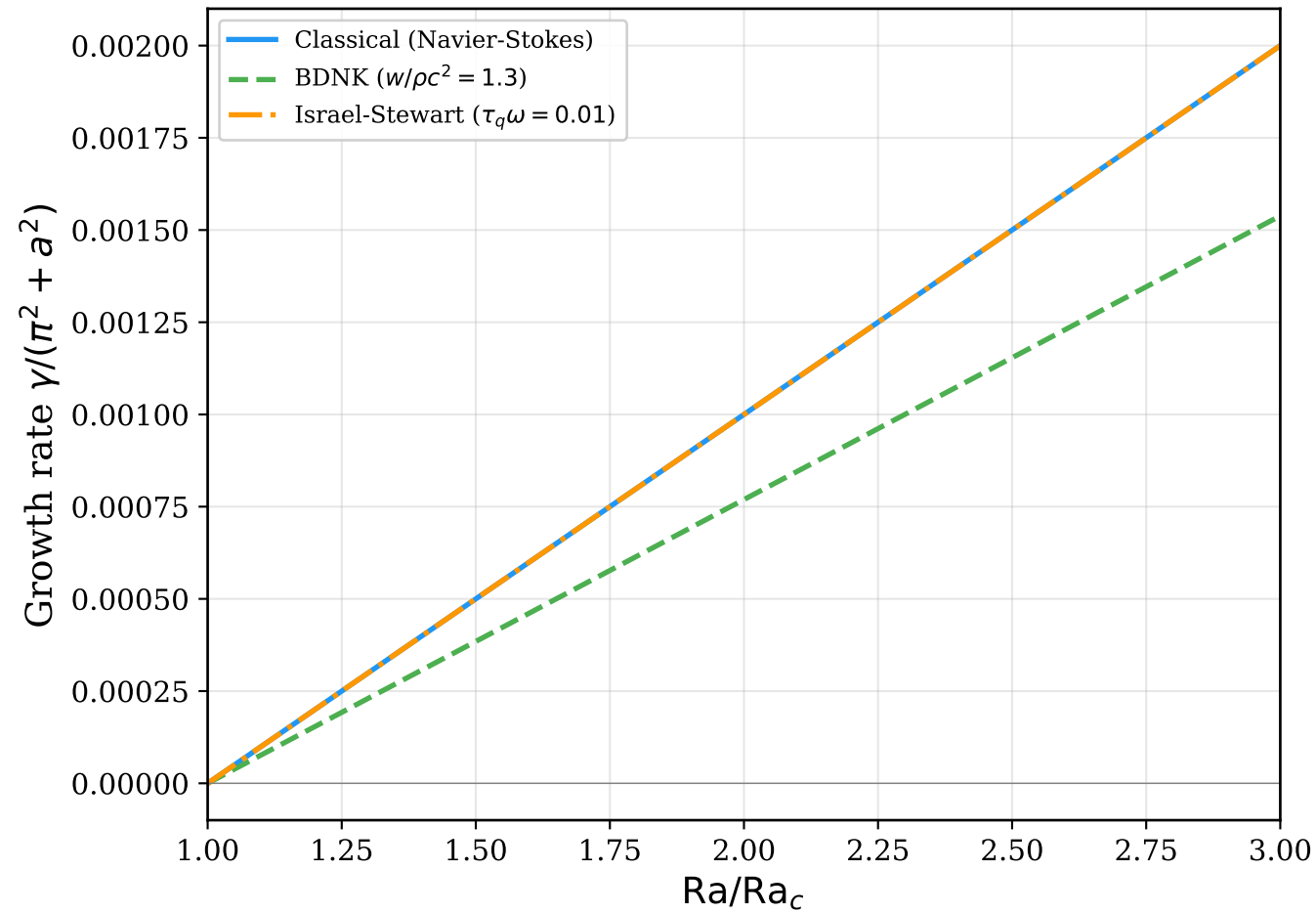
(a) Growth rates near onset ( \text{Pr} = 10^{-3} , T_1 = 10^4 )
