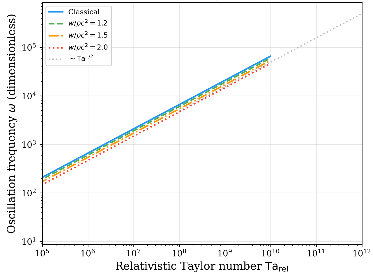
(b) Overstable frequency vs Taylor number
