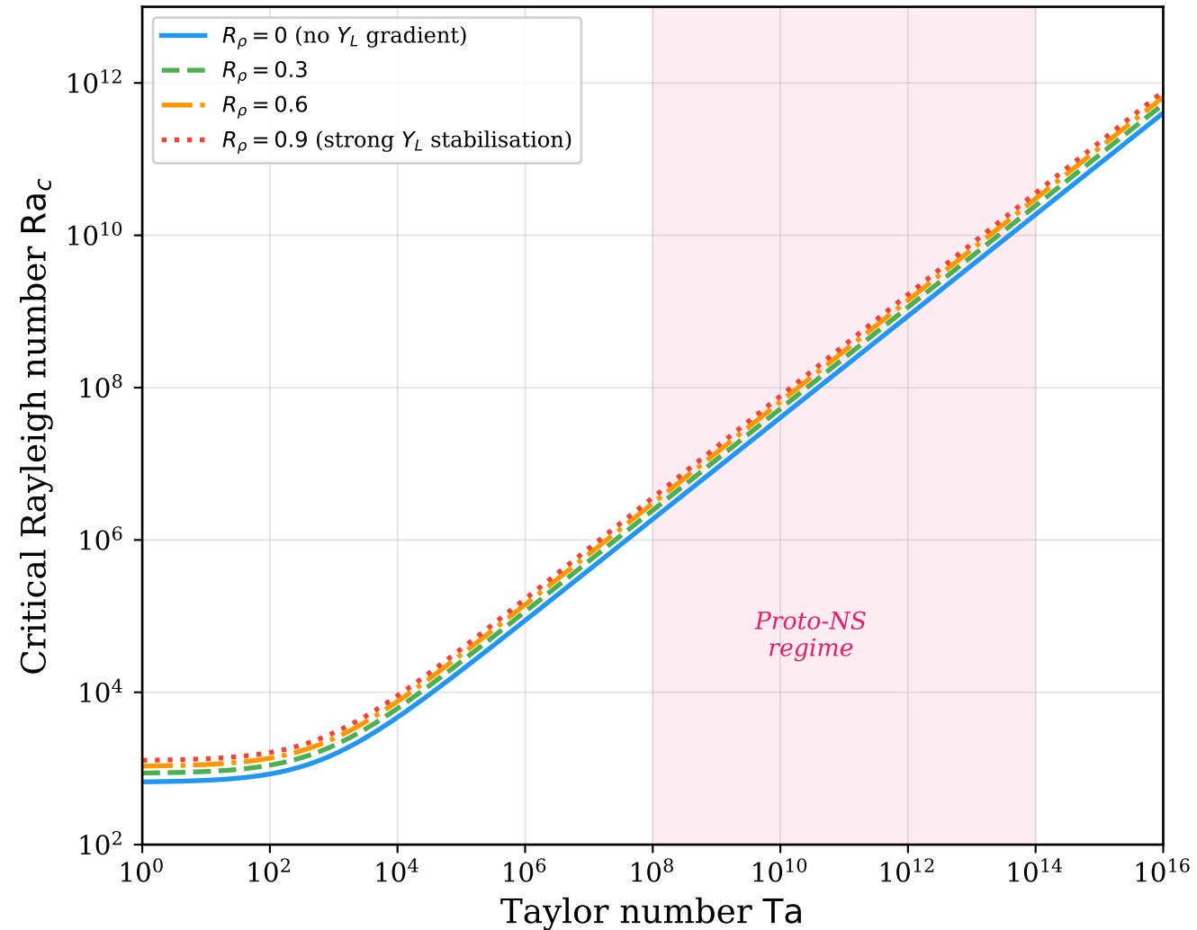
(b) Double-diffusive onset with rotation ( Le = 50 )
