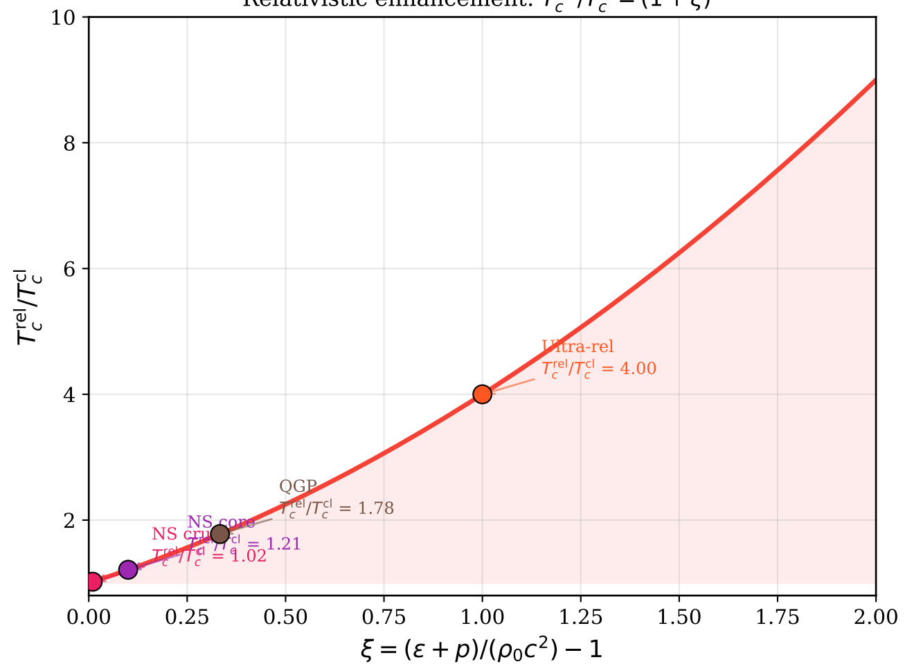
Relativistic enhancement: T_c^{\text{rel}}/T_c^{\text{cl}} = (1 + \xi)^2
