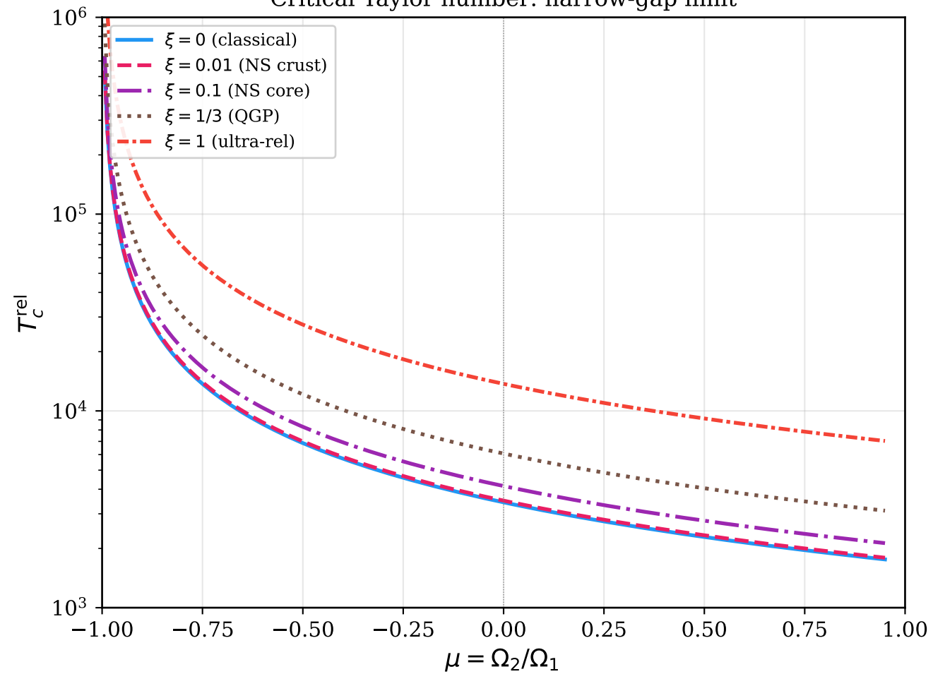
Critical Taylor number: narrow-gap limit
