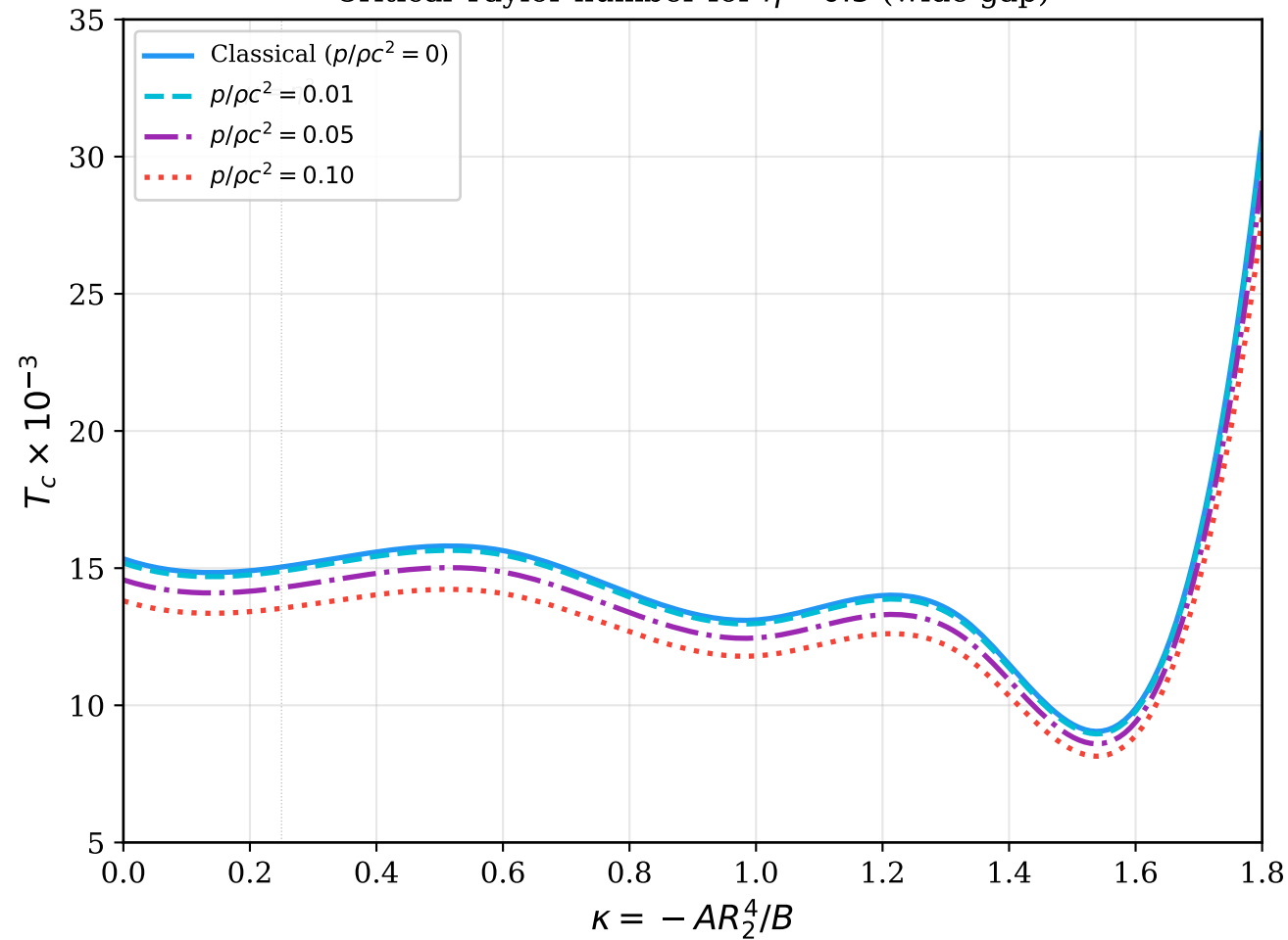
Critical Taylor number for \eta = 0.5 (wide gap)
