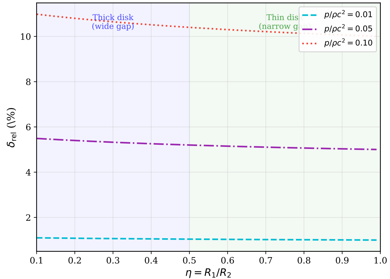
Relativistic correction \delta_{\text{rel}} vs gap ratio
