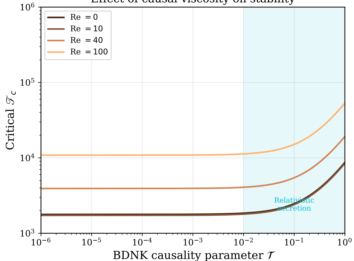
Effect of causal viscosity on stability
