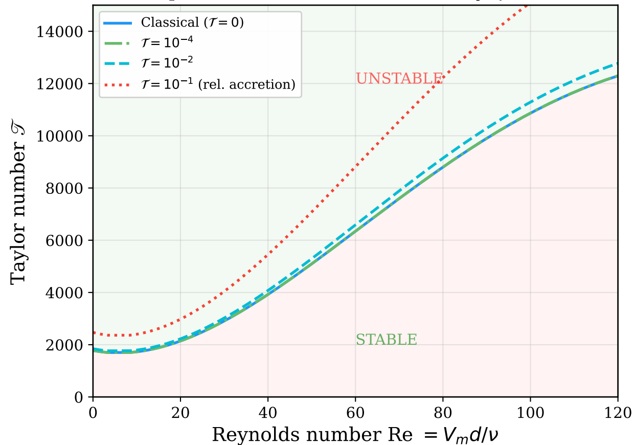
Spiral Poiseuille-Couette stability ( \mu > 0 )
