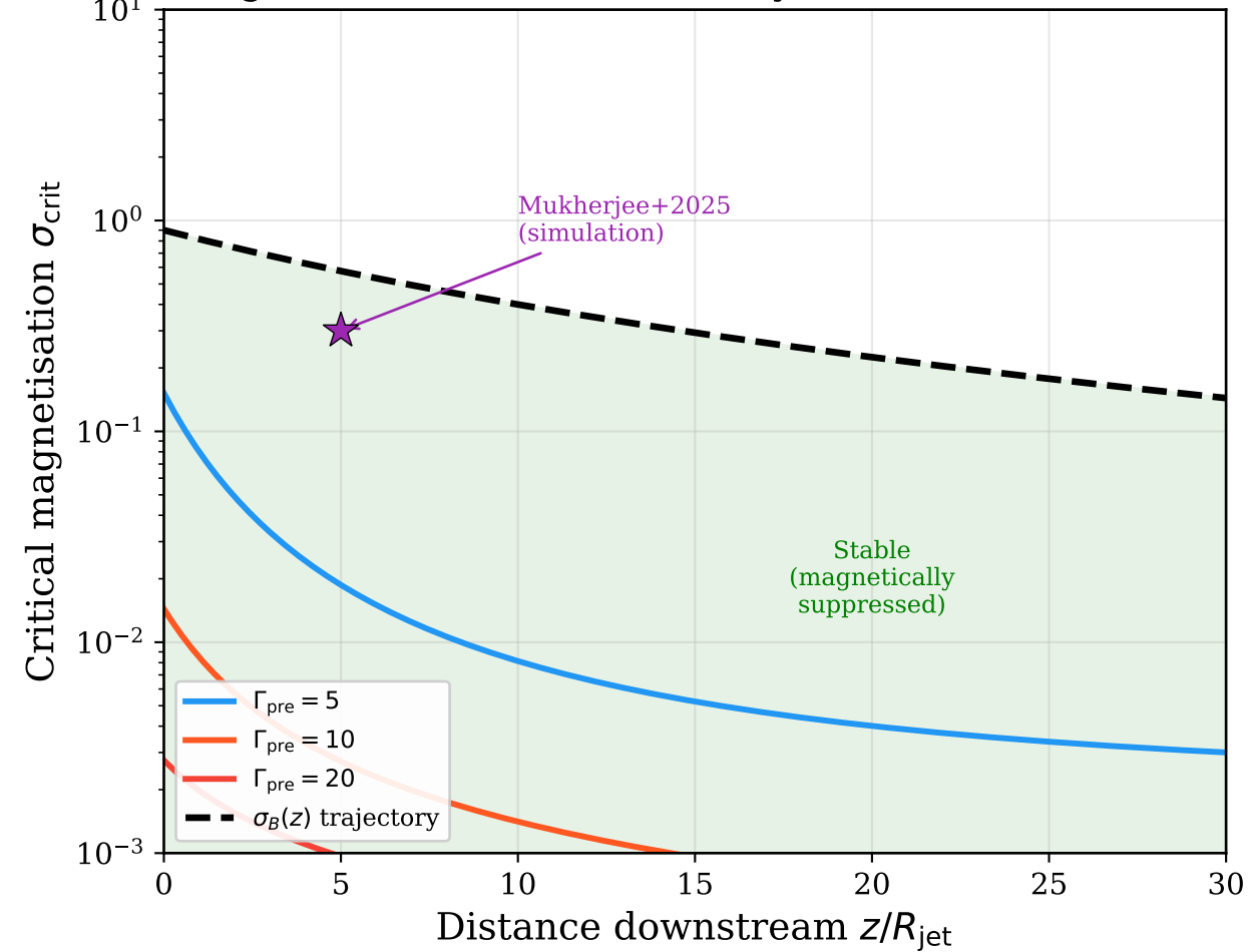
Magnetic stabilisation boundary downstream of shock
