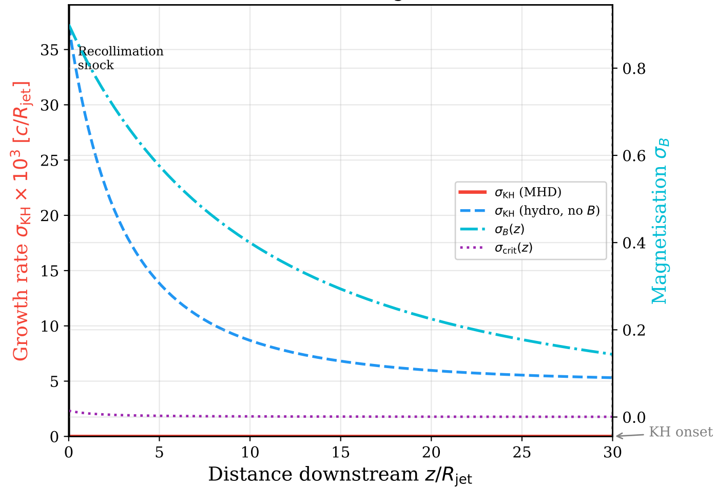
Post-recollimation KH growth rate
