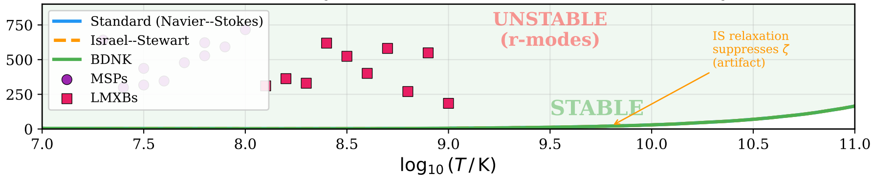
R-mode instability window: BDNK vs IS vs standard viscosity
