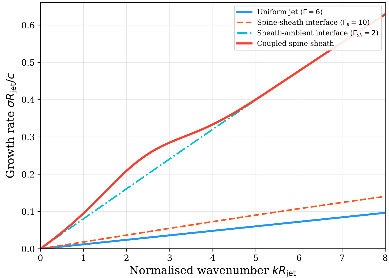
KH growth rate: spine-sheath vs uniform jet
