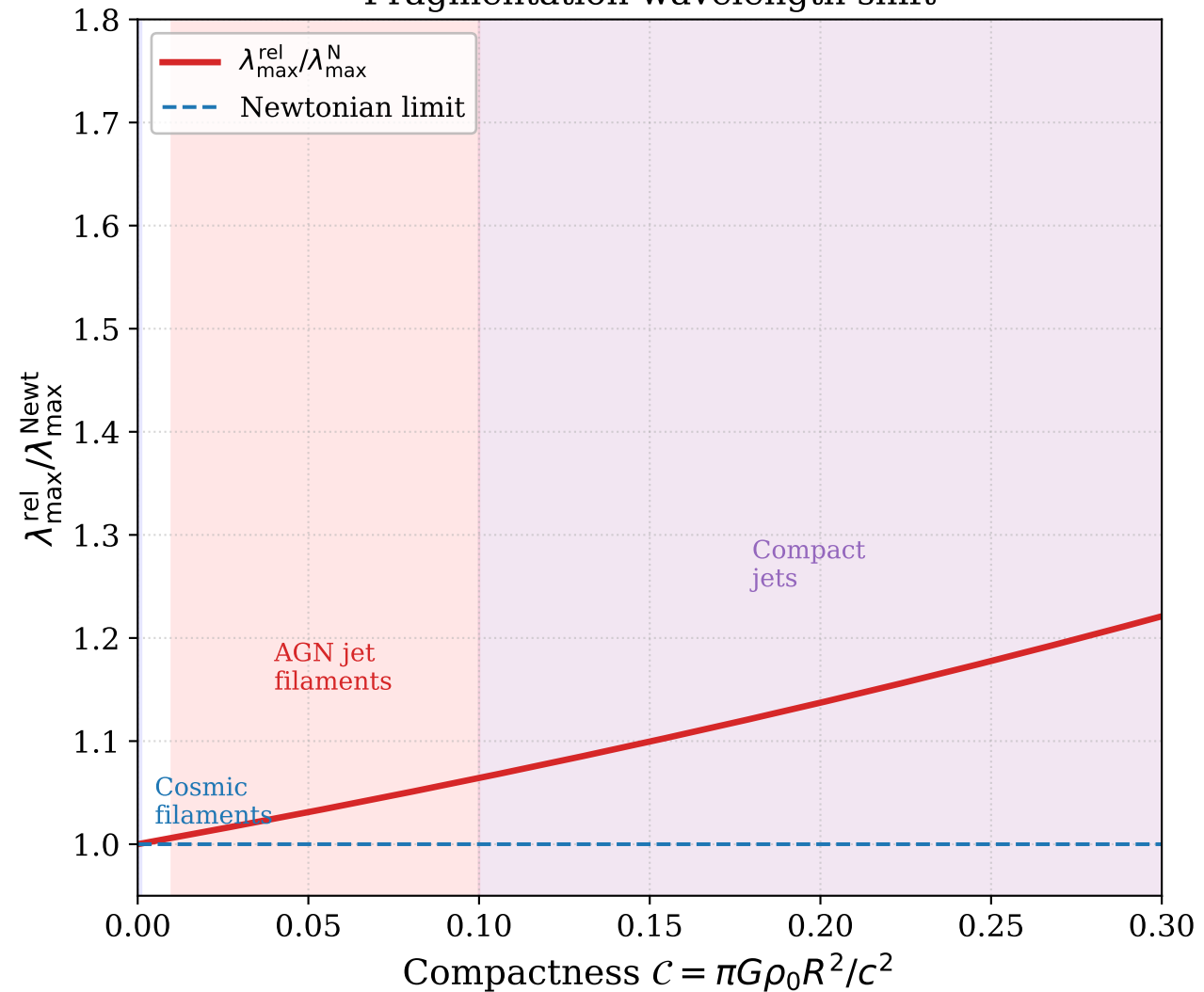
Fragmentation wavelength shift
