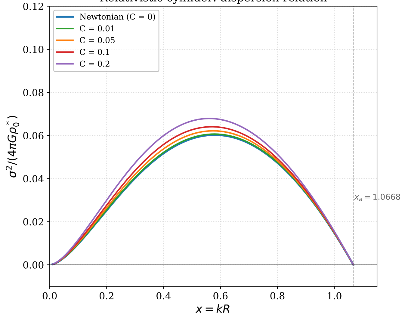
Relativistic cylinder: dispersion relation
