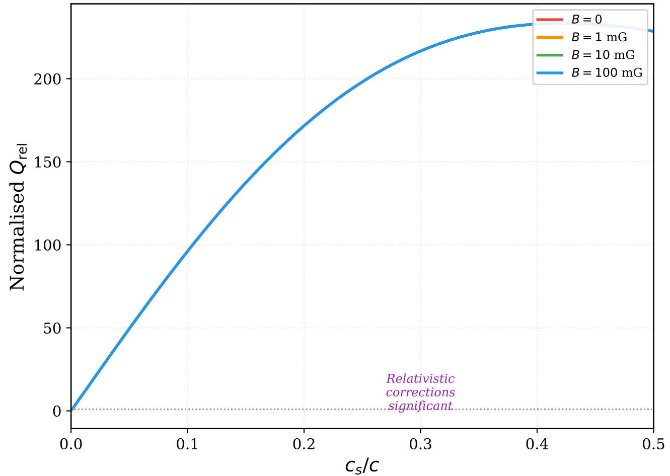
Relativistic Q vs sound speed (compact disk)
