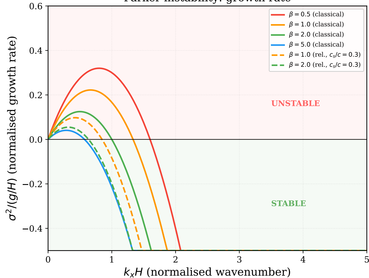
Parker instability: growth rate
