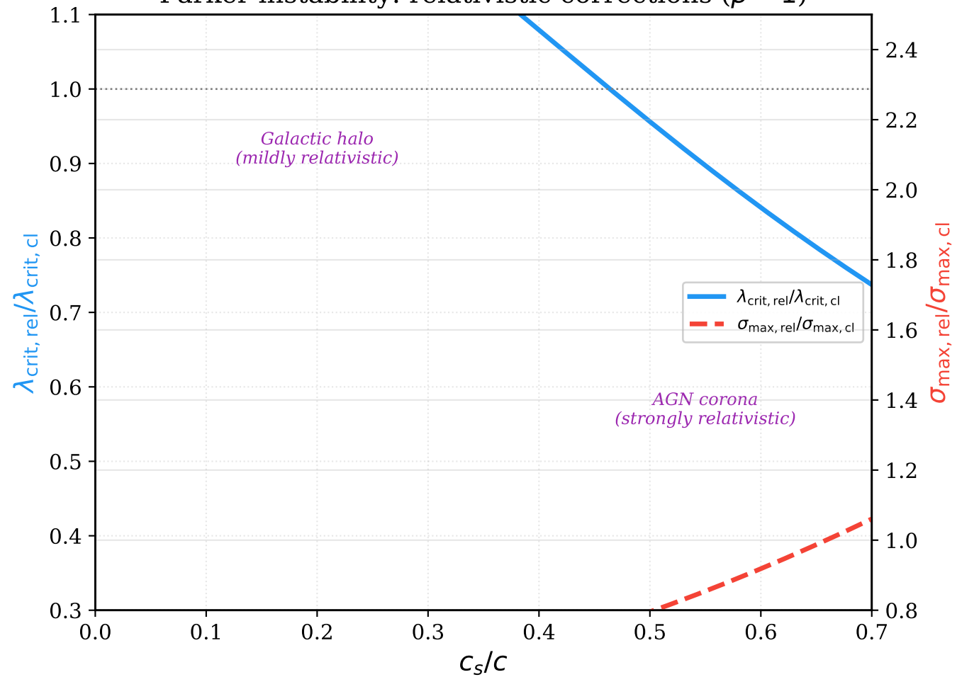
Parker instability: relativistic corrections ( \beta = 1 )
