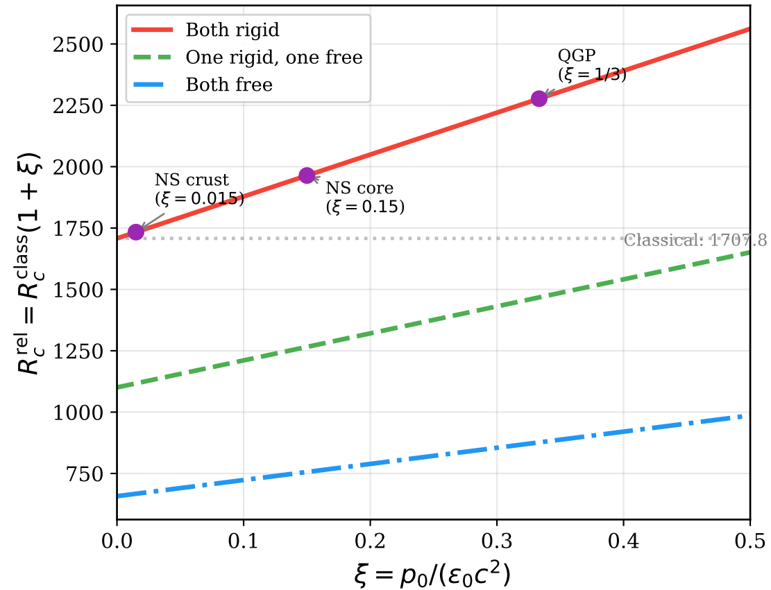
(a) Critical Rayleigh number vs. compactness
