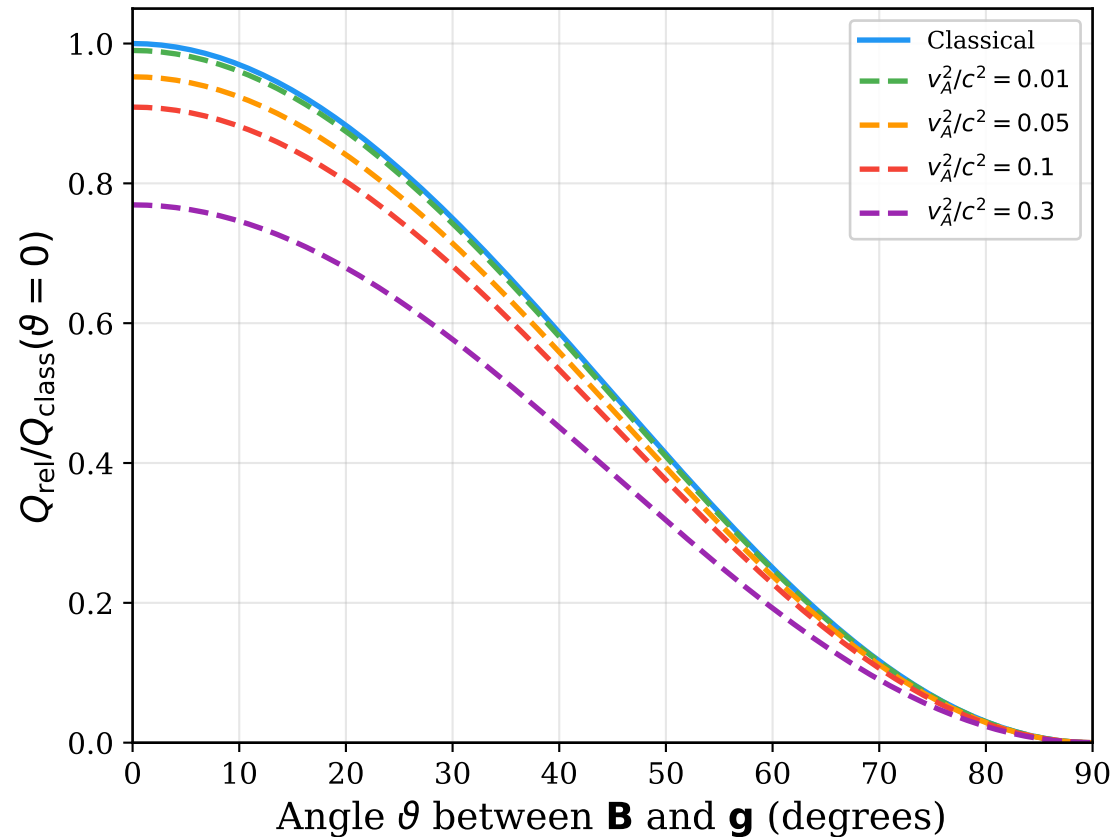
Effective Chandrasekhar number vs field inclination
