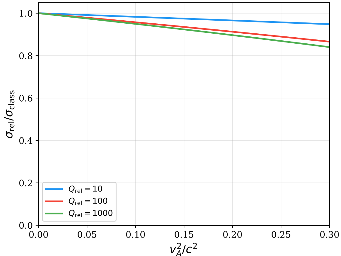
Overstable frequency shift ( \vartheta = 45^\circ )
