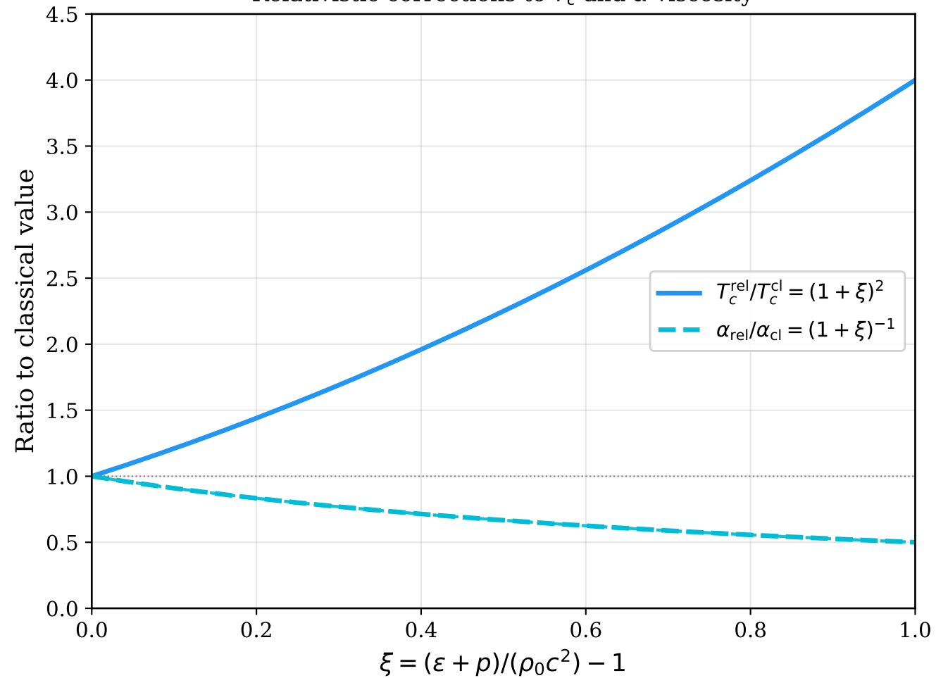
Relativistic corrections to T_c and \alpha -viscosity
