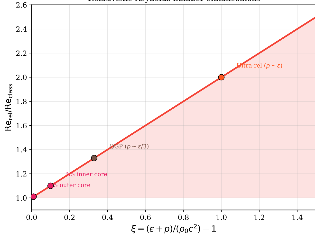
Relativistic Reynolds number enhancement
