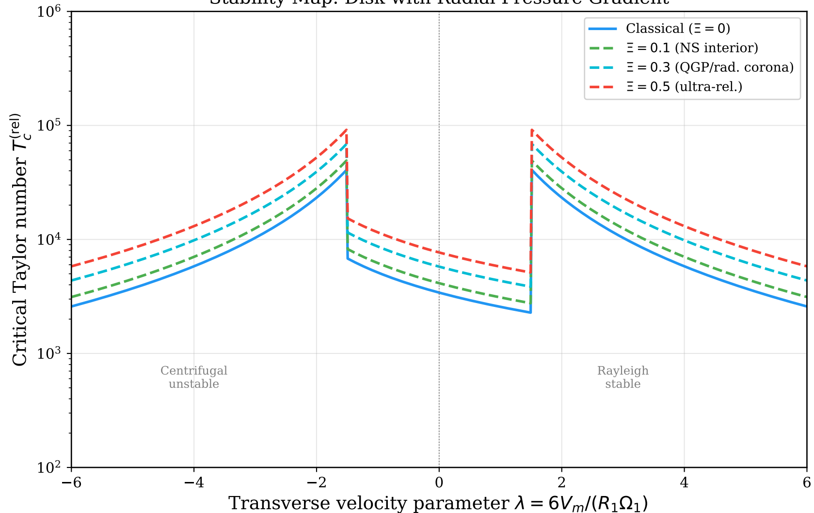
Stability Map: Disk with Radial Pressure Gradient
