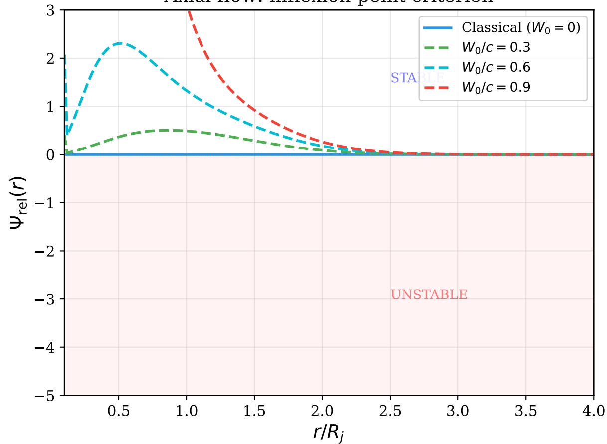
Axial flow: inflexion-point criterion
