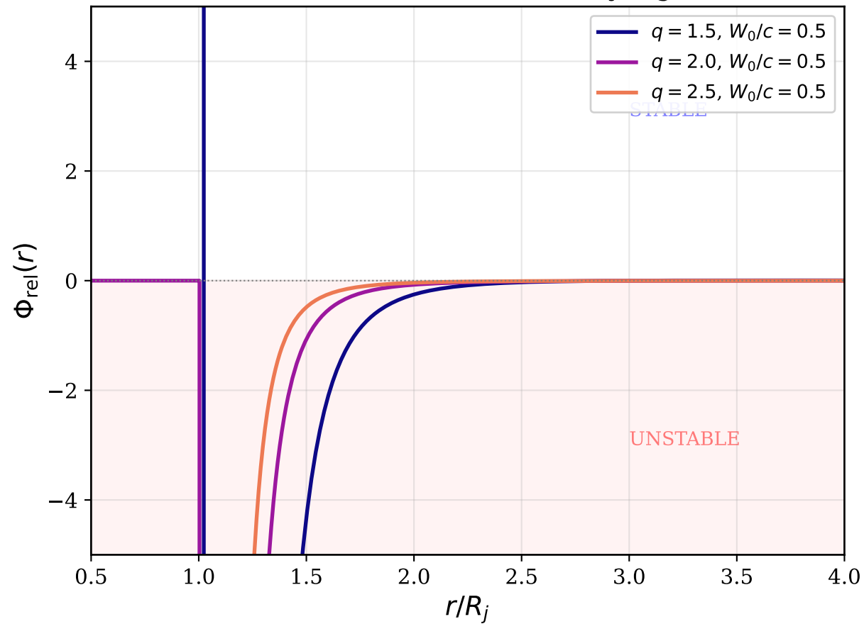
Rotation + axial flow: relativistic Rayleigh criterion
