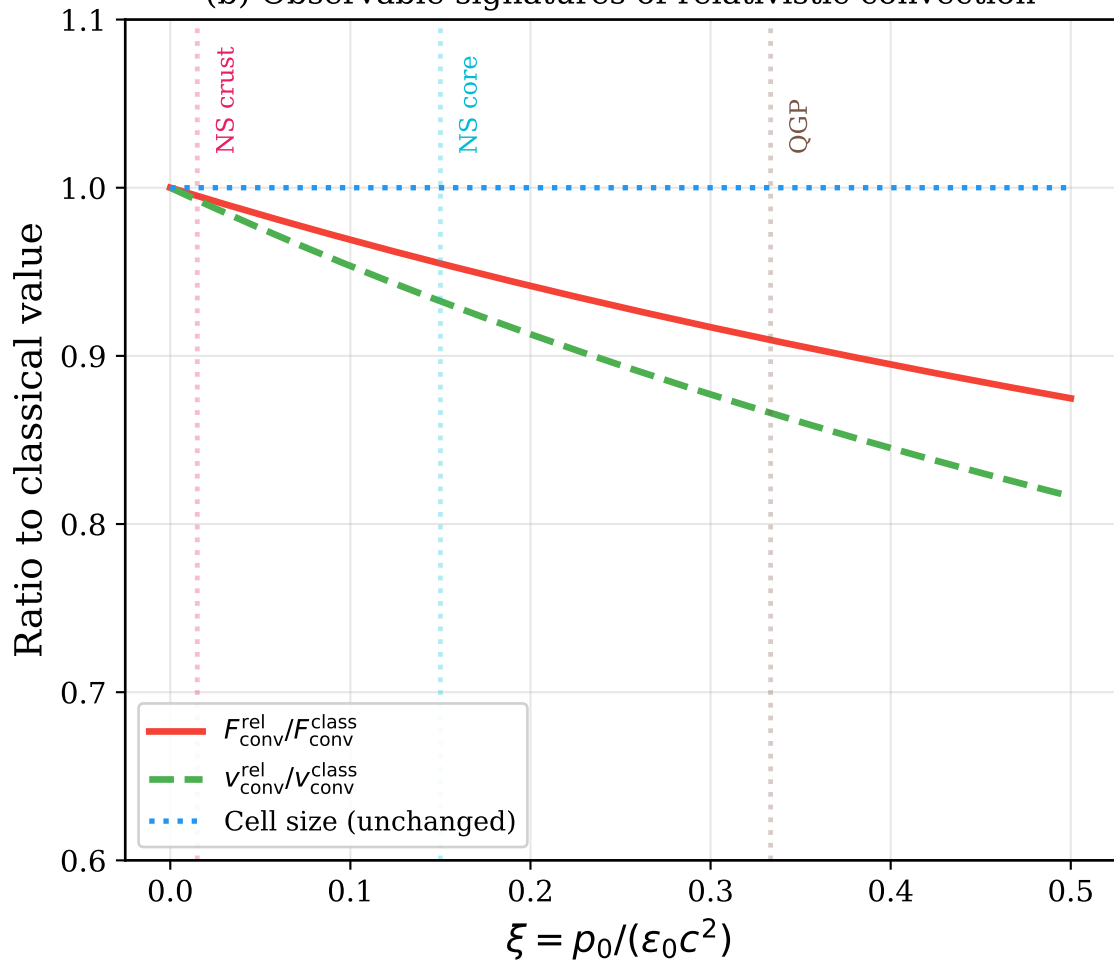
(b) Observable signatures of relativistic convection
