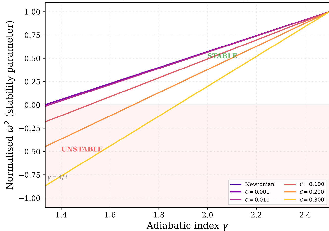
Stability boundary shift with compactness
