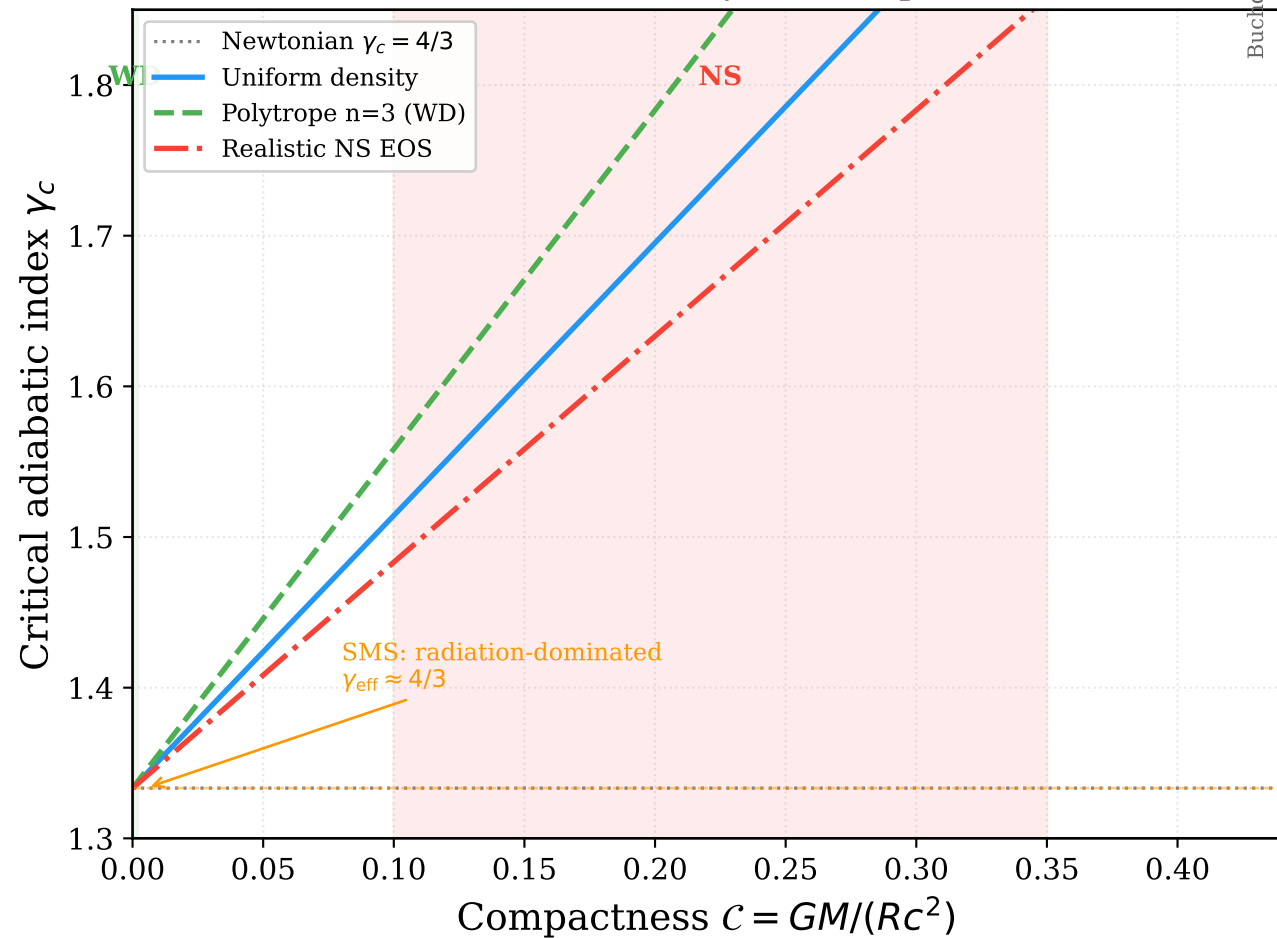
GR destabilisation: \gamma_c vs compactness
