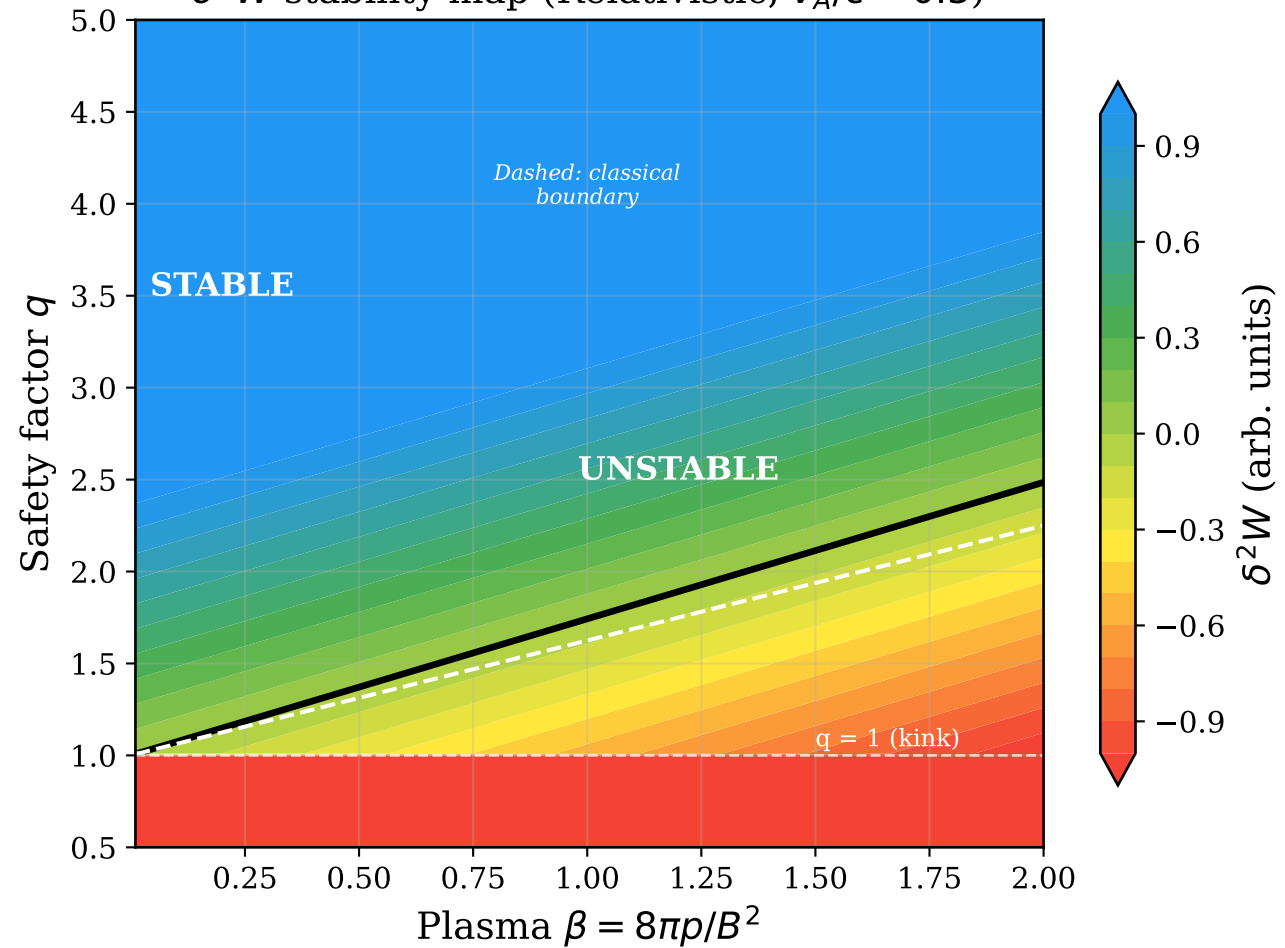
\delta^2 W stability map (Relativistic, v_A/c = 0.3 )
