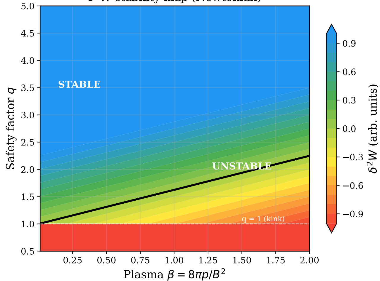
\delta^2 W stability map (Newtonian)
